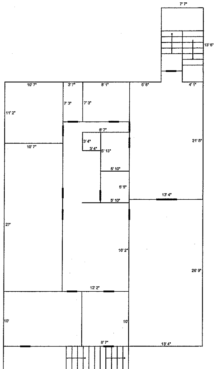
1ST FLOOR
