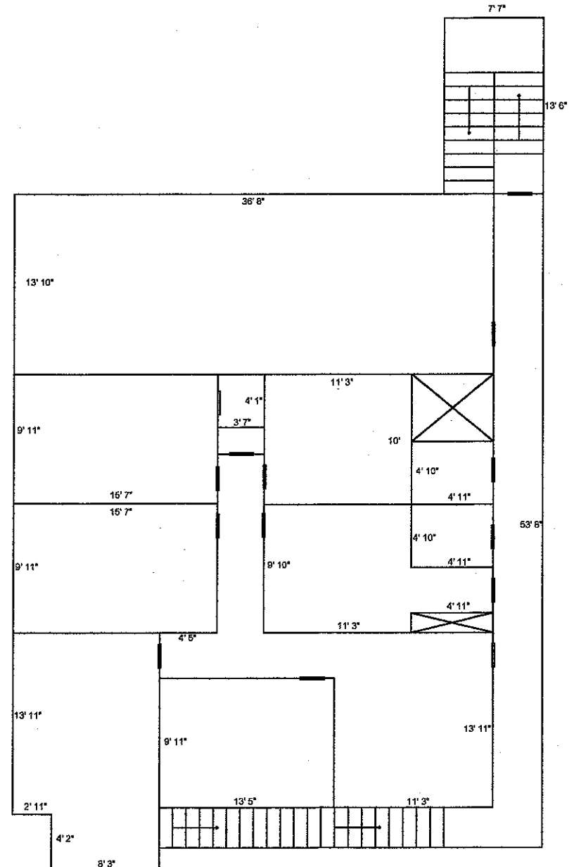
2ND FLOOR
