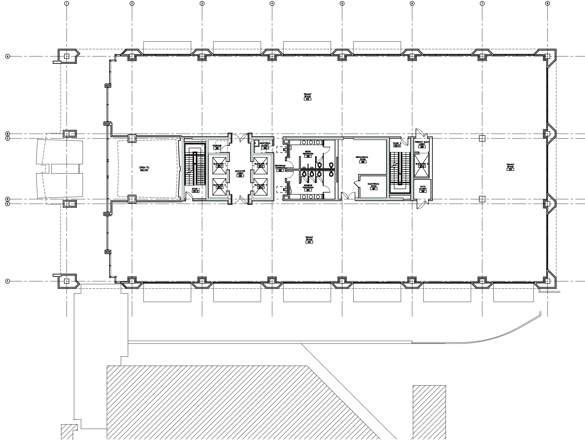
1 LEVEL 02
