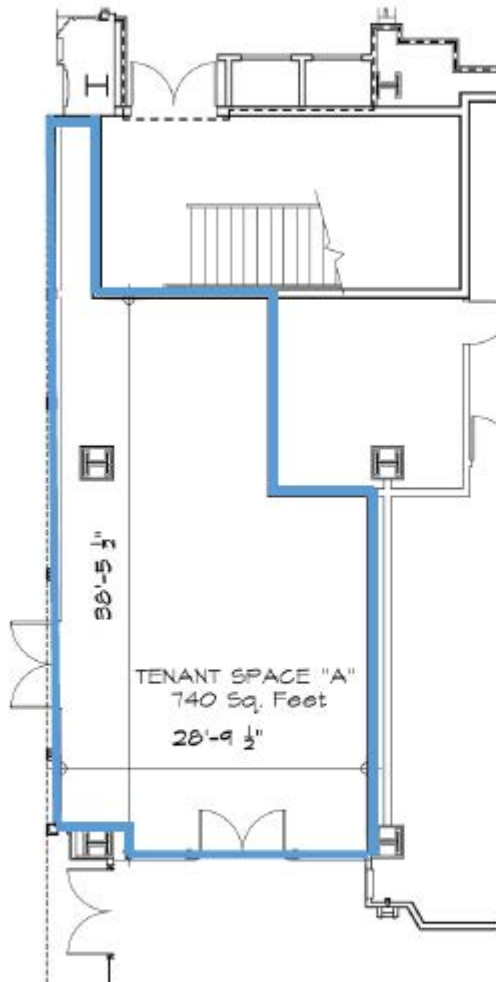
1 FLOOR PLAN
