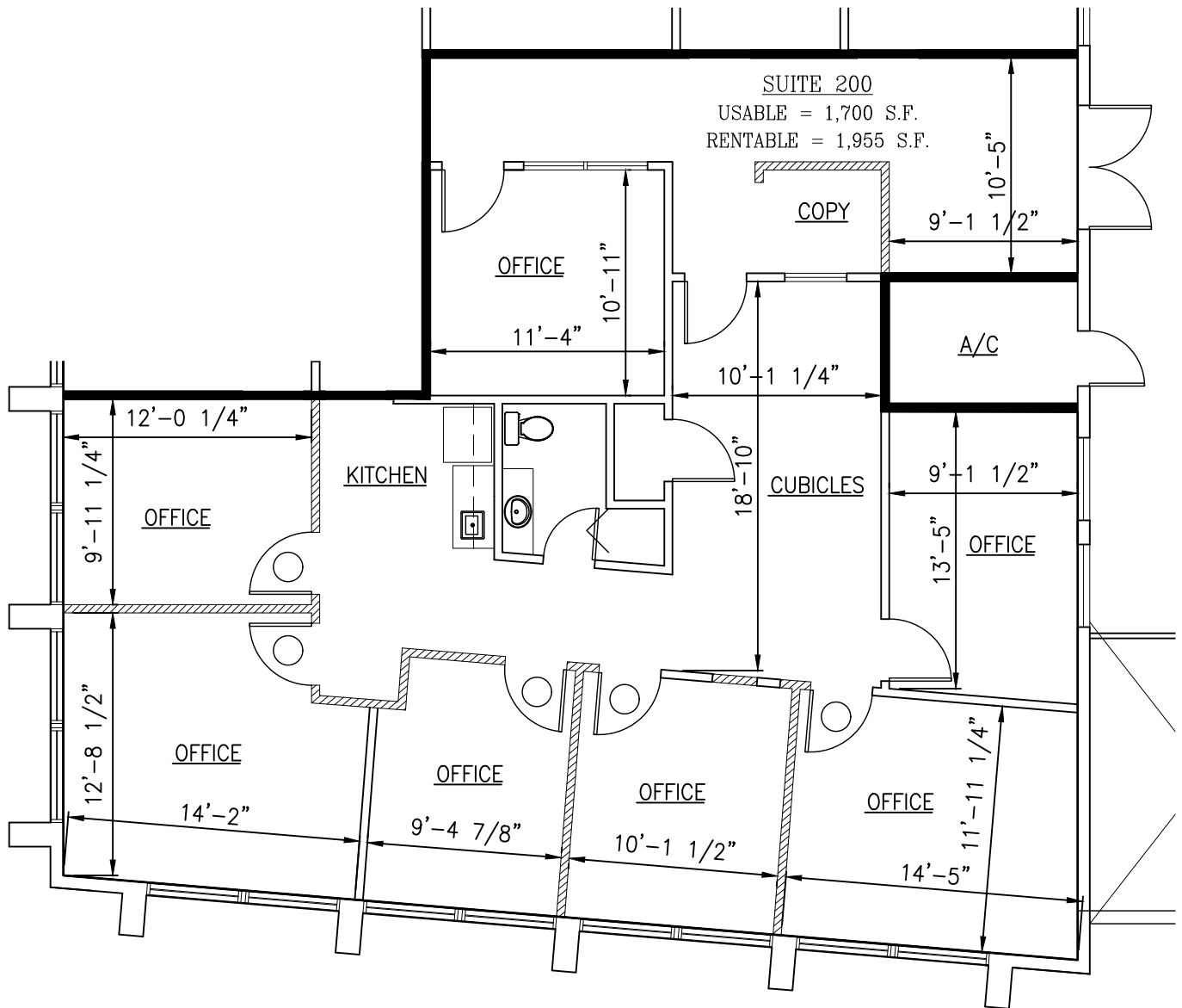
1 SUITE 200 FLOOR PLAN SCALE: 1/8"=1'-0"
