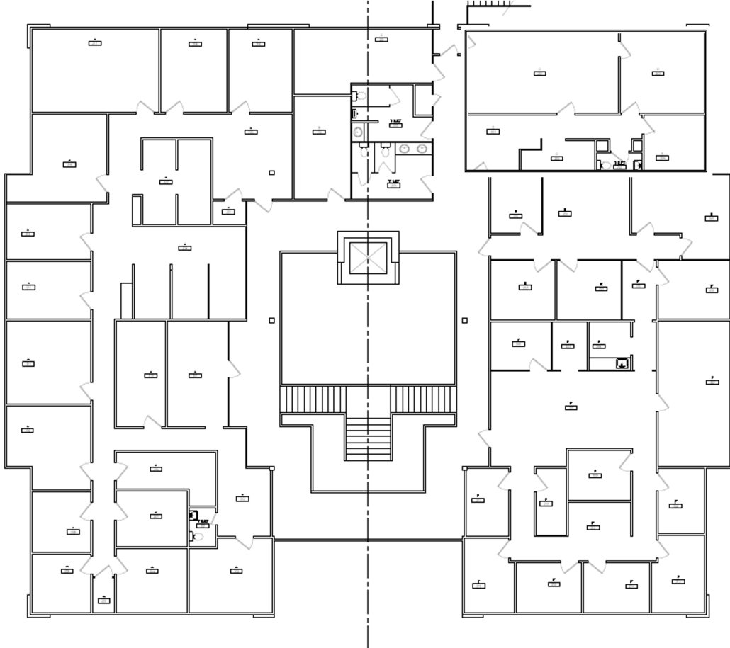
1 EXISTING 2ND FLOOR FLOOR PLAN
