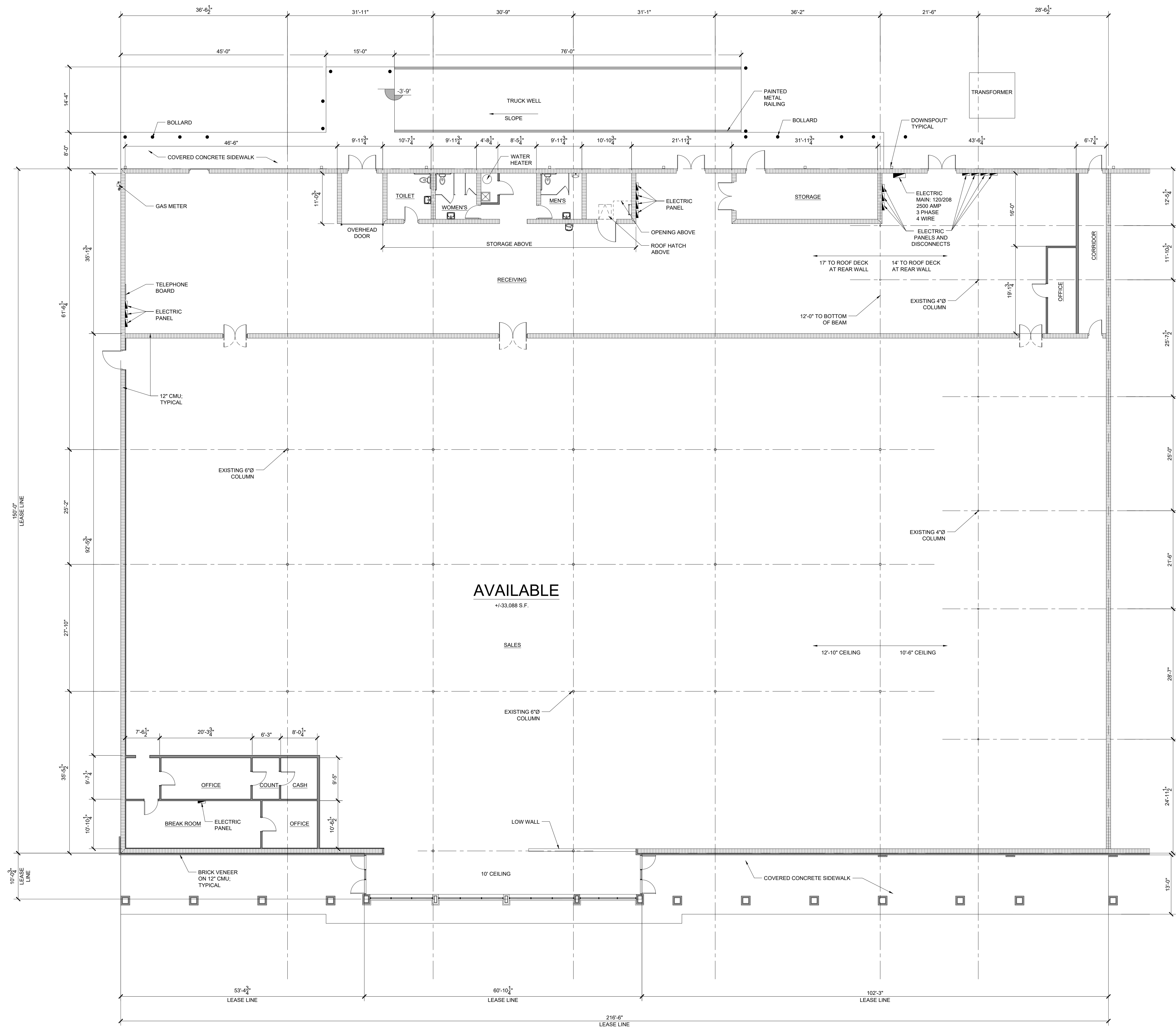
1 FLOOR PLAN LOD SCALE: 3/32" = 1'-0"
