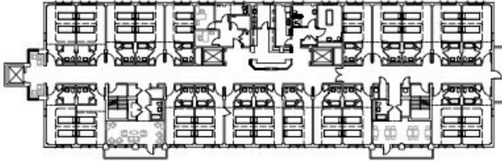
3 3RD FLOOR FURNITURE PLAN
