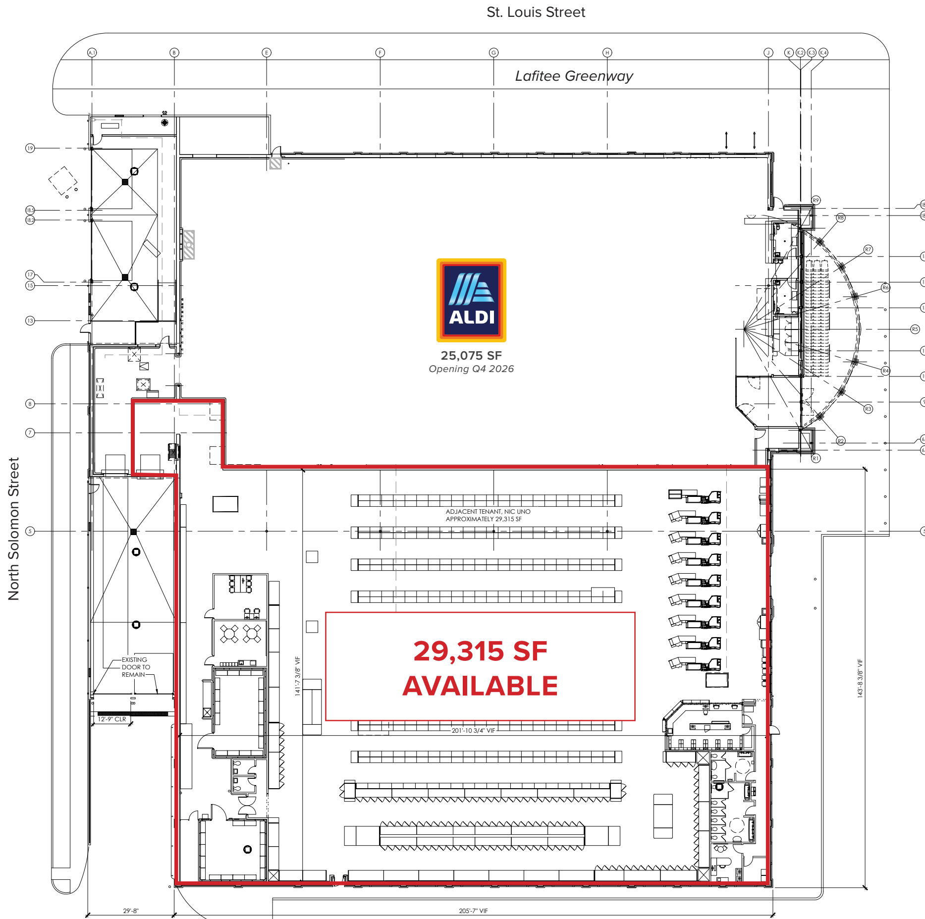
1 Concept Floor Plan SCALE: 1/16" = 1'-0"
