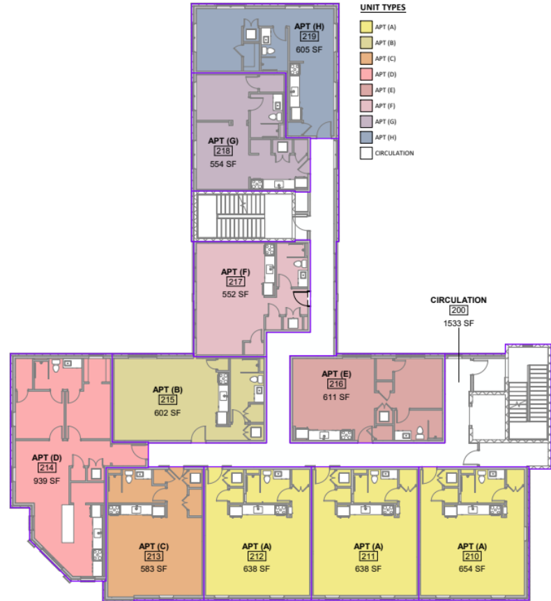
2 2nd FLOOR UNIT PLAN G2.1 1" = 10'-0"
