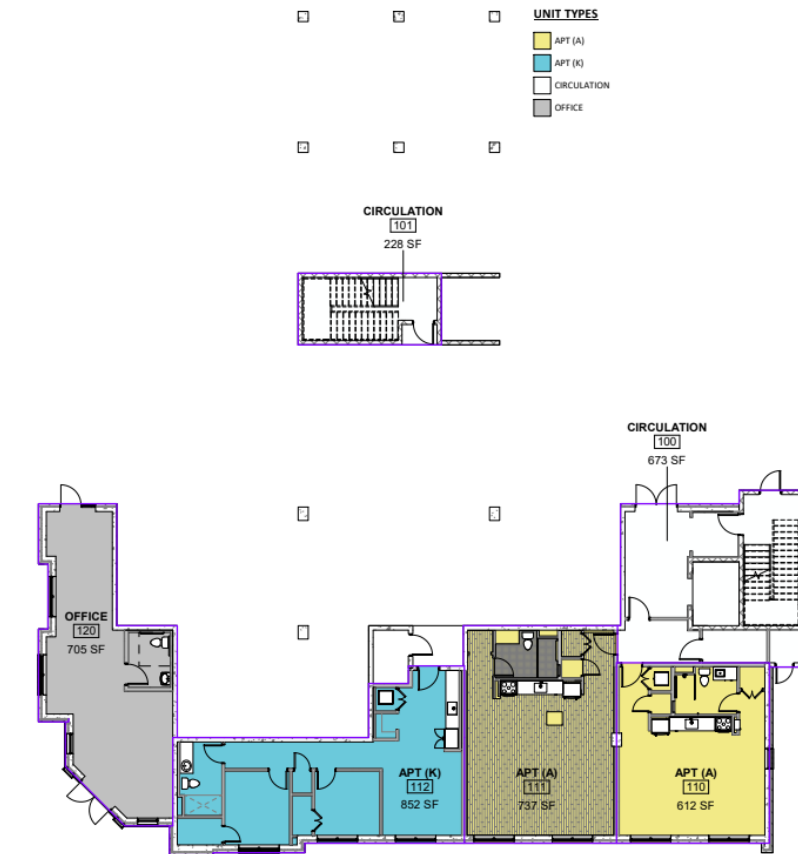
1 1st FLOOR UNIT PLAN G2.1 1" = 10'-0"
