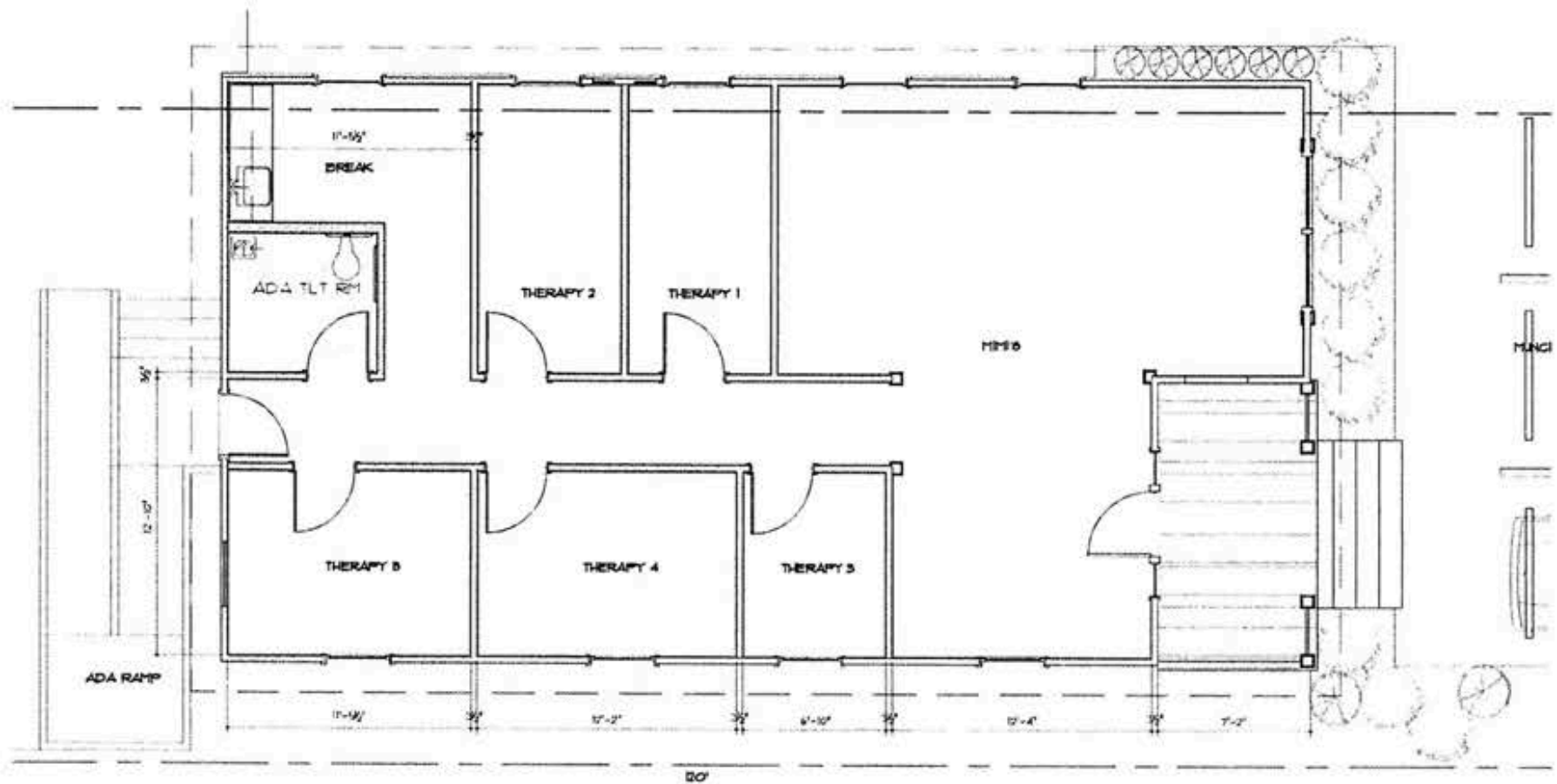
2 FLOOR PLAN
