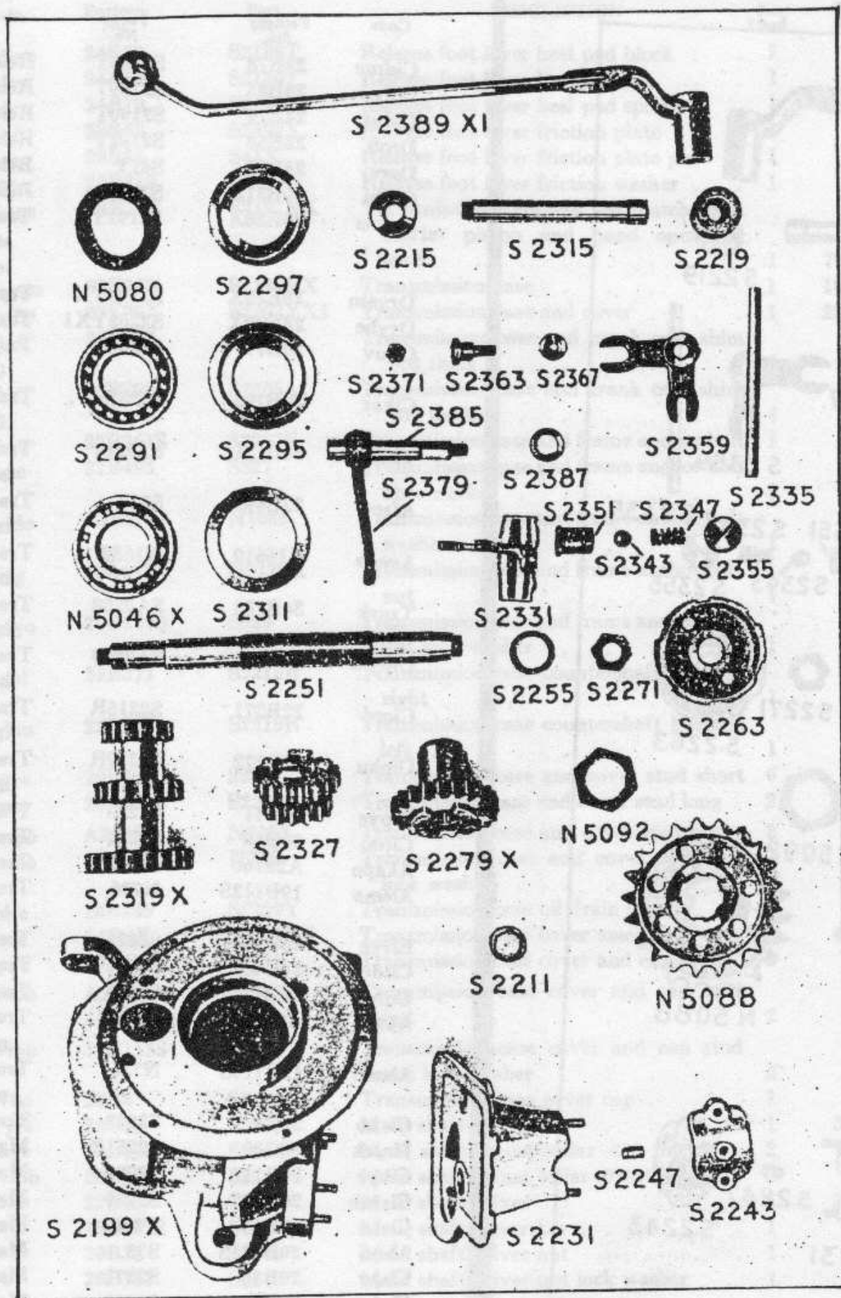
Transmission Group
