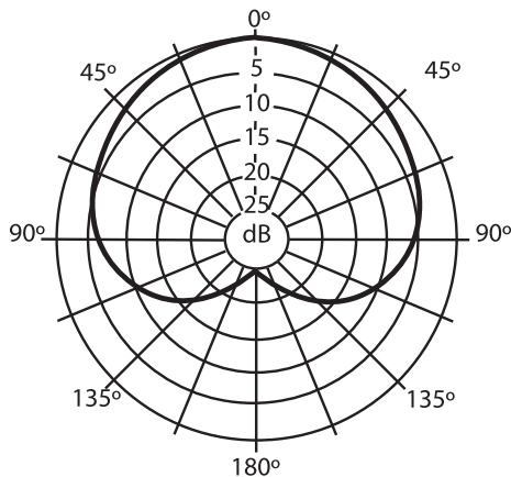
C02H Polar Pattern
