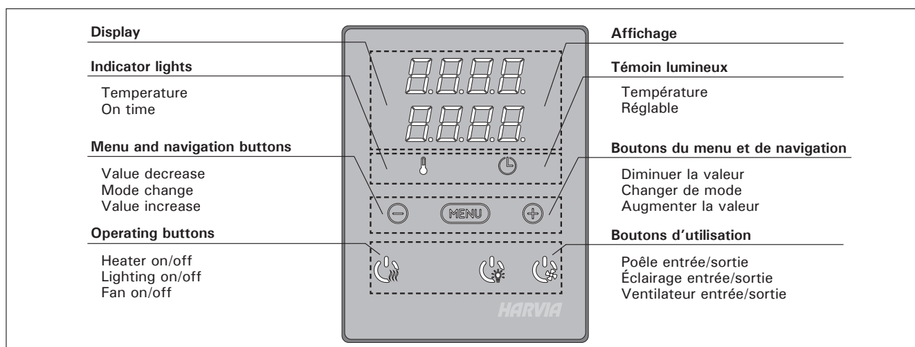
Figure 2. Control panel
