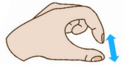
Pinch-to-zoom
