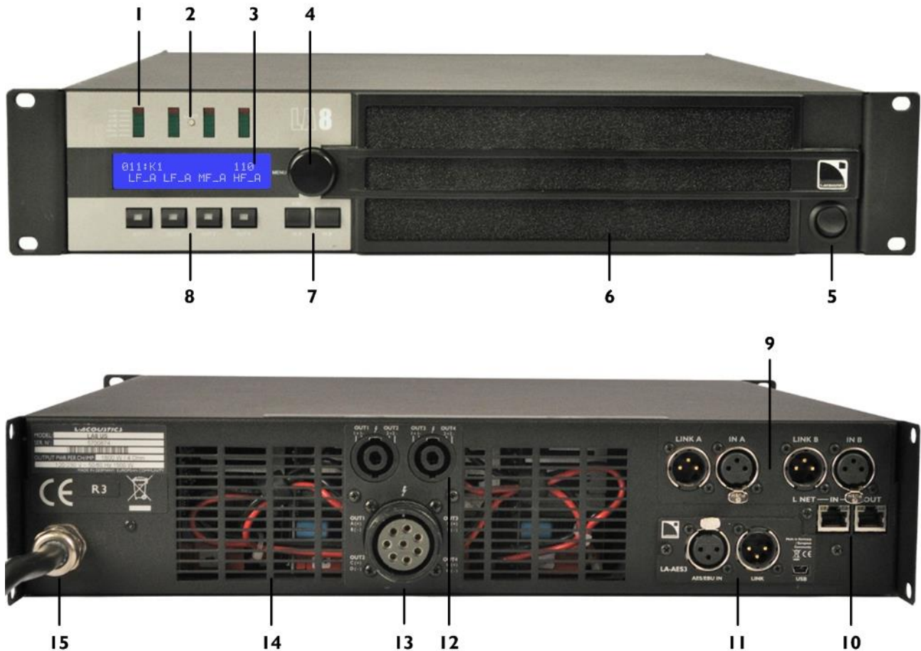
Figure 2: LA8 front and rear panels
