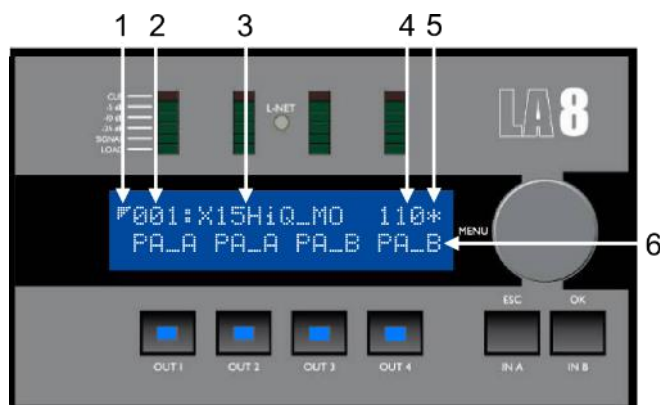
Figure 15: Main screen
