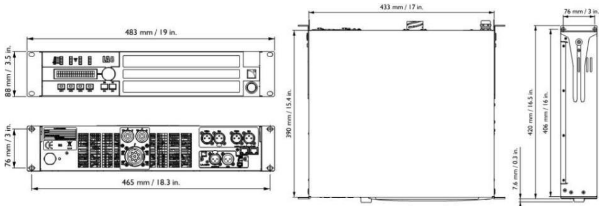
Figure 5: LA8 dimensions
