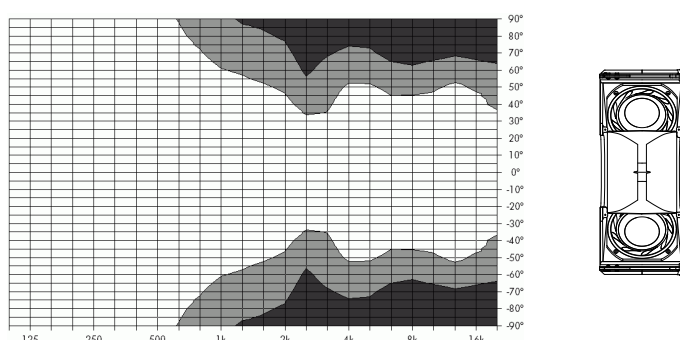
Fig. 10: Isobar diagram T10 point source, horizontal
