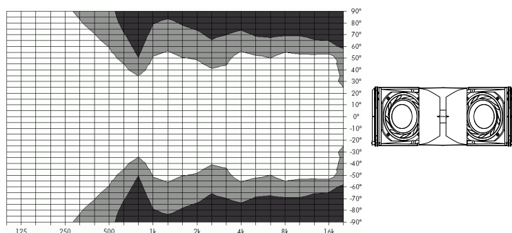
Fig. 8: Isobar diagram T10 line source, horizontal
