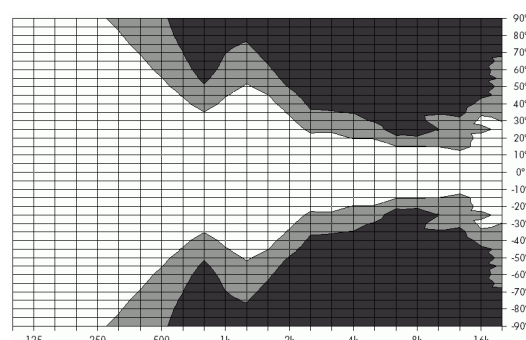
Fig. 11: Isobar diagram T10 point source, vertical
