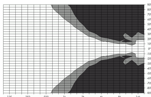
Fig. 9: Isobar diagram T10 line source, vertical
