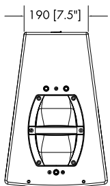
V7P/V10P cabinet dimensions in mm [inch]
