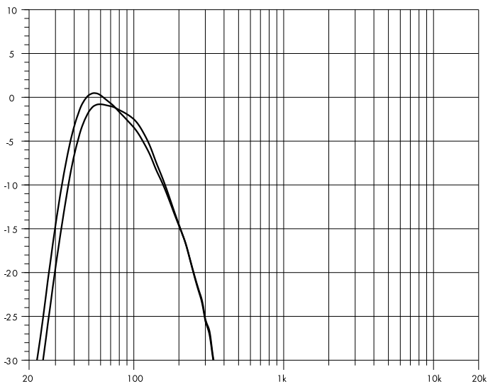
XSL-SUB frequency response, Fln setup - Standard and 100 Hz mode
