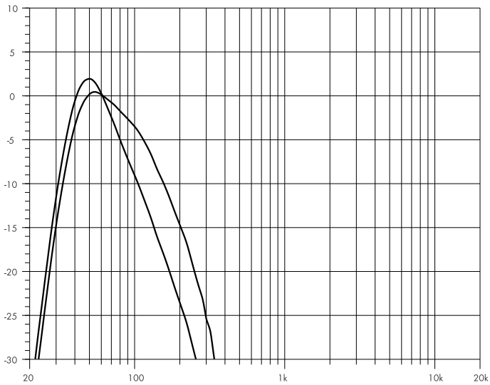
XSL-SUB frequency response, Standard and INFRA modes
