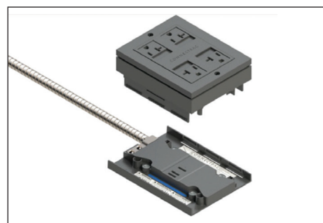
Receptacle Device snaps into the Express Power Hub, Power Hub is attached to a prewired, flexible conduit.
