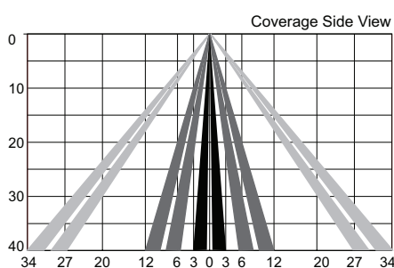
HBL4 Coverage Side View
