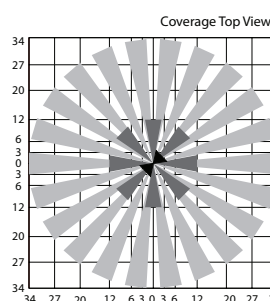
HBL4 Coverage Top View
