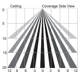
HBL3 Coverage Side View
