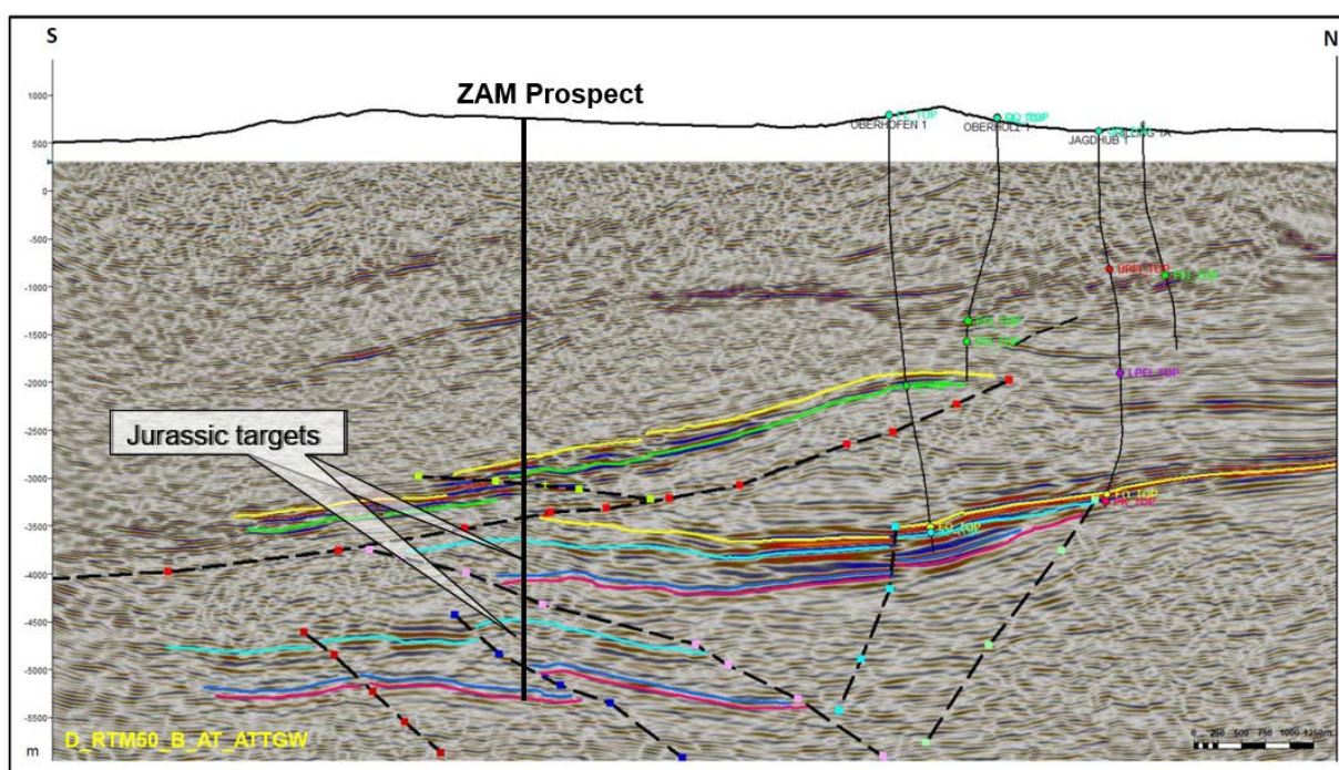
Seismic cross section of Large ZAM prospect
