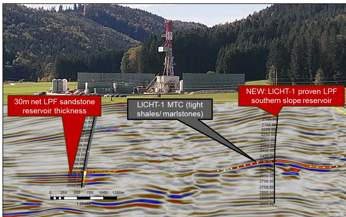
The RED Drilling & Services GmbH (RED) E-202 drilling rig at the LICHT-1 well location, 3D seismic & well results. (Note: MTC is Mass Transport Complex)
