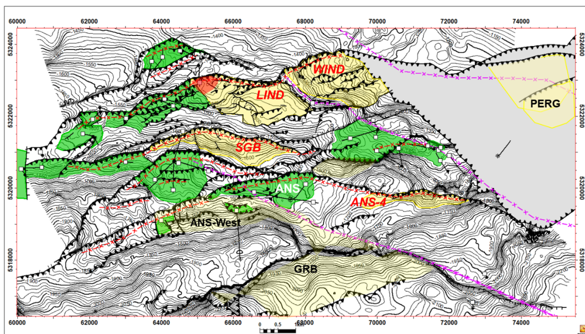
Map showing Anshof Near Field Exploration prospects in the ADX-AT-II licence in Upper Austria. Prospects and appraisal structures named in red are located close to the Anshof permanent production facility (PPF), i.e. ANS-4, SGB, LIND & WIND are appraisal projects. Existing oil fields are coloured in green
