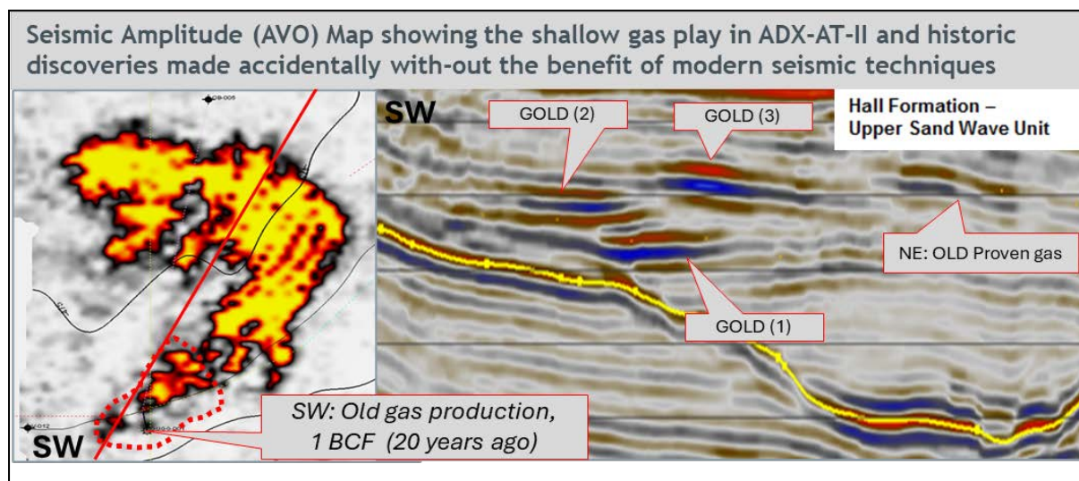
3D Seismic and Map showing new shallow gas prospects, already partly proven by old wells
