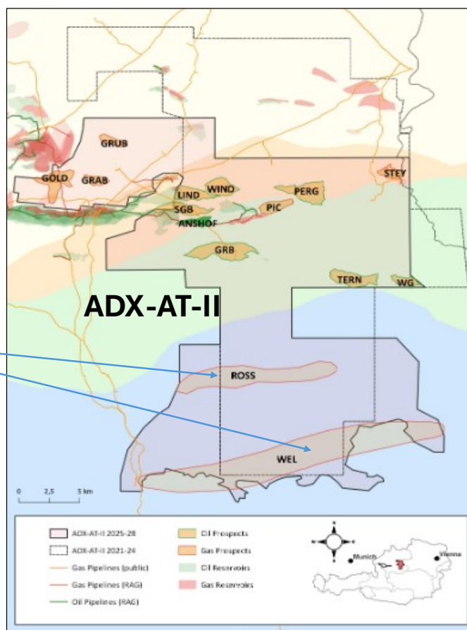
The Welchau play and the Rossberg prospect within the revised ADX-AT-II licence area
