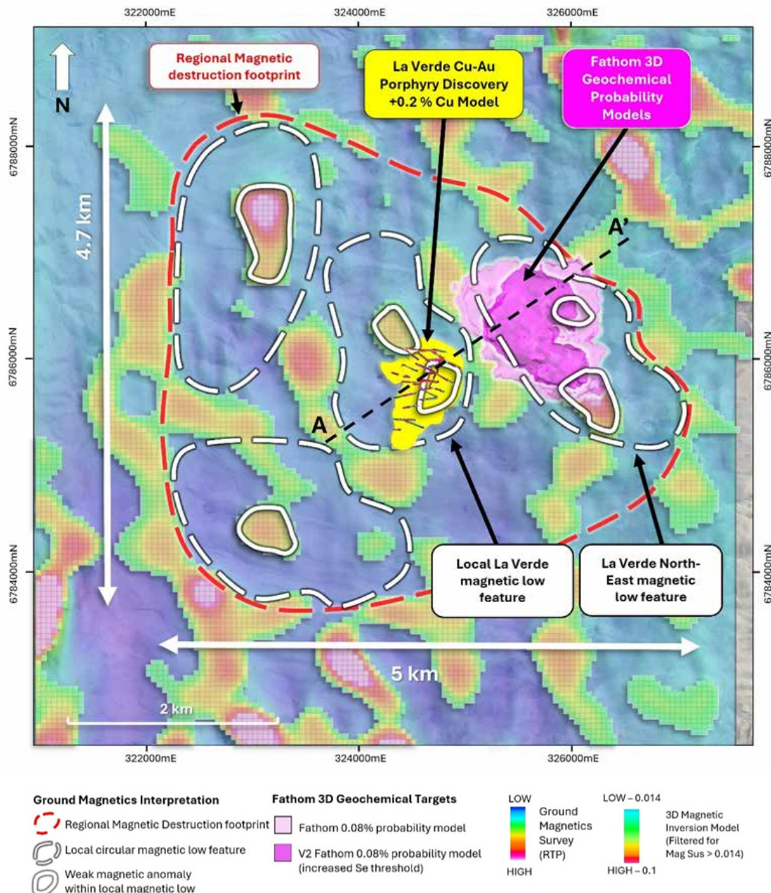
Figure 2: Plan view showing the La Verde +0.2% Cu mineralisation interpolant in relation to regional magnetic destruction footprint (red dashed), local magnetic low features (white dashed), weakly magnetic anomalies (white line) and Fathom 3D geochemical probability models (purple isosurfaces). Left - shown overlain on reduced-to-the-pole (RTP) ground magnetics and the 3D magnetic inversion model (sliced at 850 RL, displayed as blocks, filtered for Magnetic Susceptibility > 0.014).
