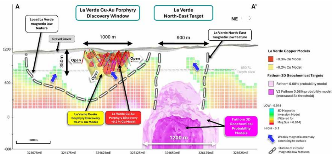
Figure 3: Long section view A - A' facing north-west showing the La Verde +0.2% (yellow) and +0.3% copper (red) mineralisation interpolants in comparison to the 3D magnetic inversion model (displayed as blocks, filtered for Magnetic Susceptibility > 0.014) and 3D geochemical target at La Verde North-East. Local circular magnetic low features are outlined (white dashed line) and locations where shallow weakly magnetic anomalies extend to the surface are marked with blue arrows.
