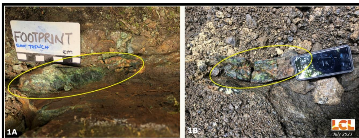
Plate 2: Examples of in-situ boudins of high-grade nickel sulphide exposed in pits/trenches. Plate 1B sample 176019: 13.4% Ni, 5.4g/t Au 4 - 10cm x 30cm boudin of nickel sulphide, garnierite, magnetite and trace molybdenite hosted in a shear striking 050 degrees.
