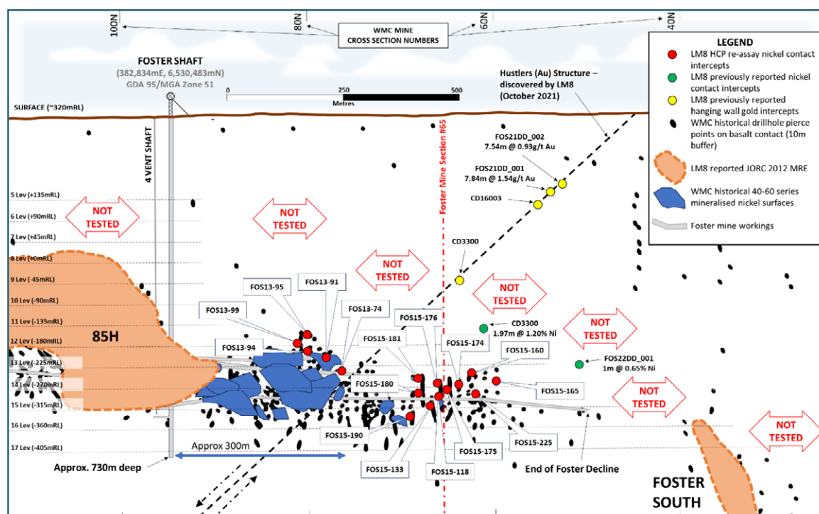
Figure 6: Long projection view of the southern end of the Foster nickel mine illustrating location of Lunnon Metals' 85H and Foster South nickel MRE areas adjacent to historical WMC mineralised areas (blue), Foster Shaft and decline and previous Company surface DD completed in 2021/2022 (view looking towards 045°, north-west to left of image).
