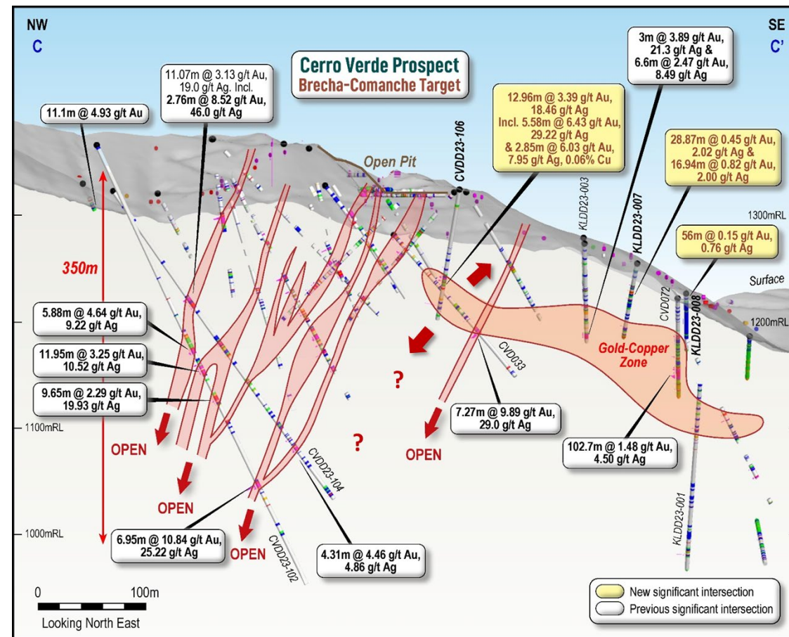
Brecha-Comanche Cross Section with Interpreted Epithermal Vein Mineralisation
