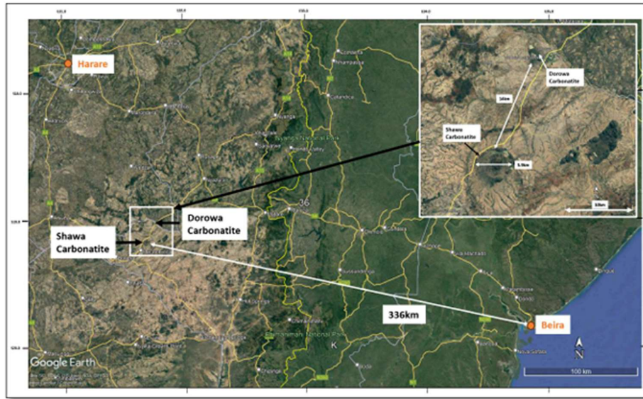
Figure 3: Shawa Carbonatite in relation to Harare and the Mozambican Beira Port shown on Google Earth image, yellow roads national tar roads. Insert of Shawa and adjacent Dorowa carbonatites.
