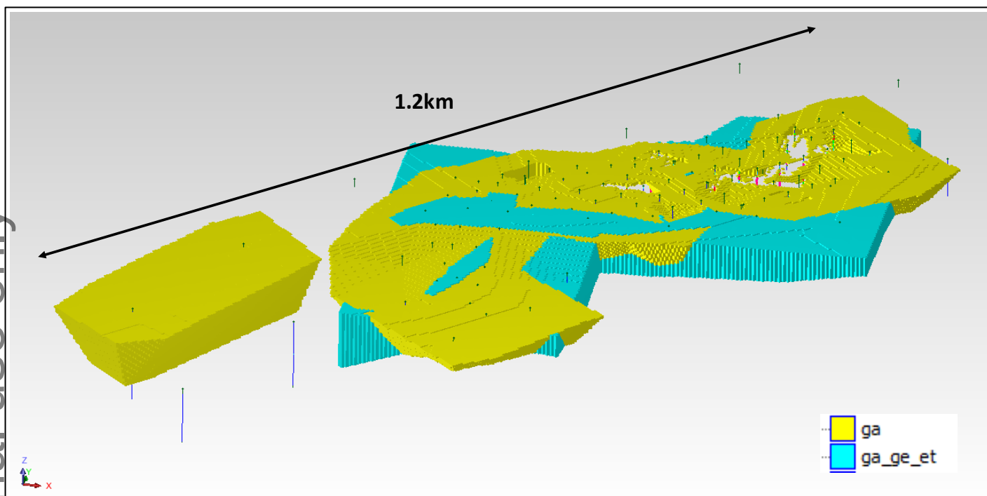
Figure 10 – Nxuu Gallium/Germanium Exploration Target – Geospatial Location
