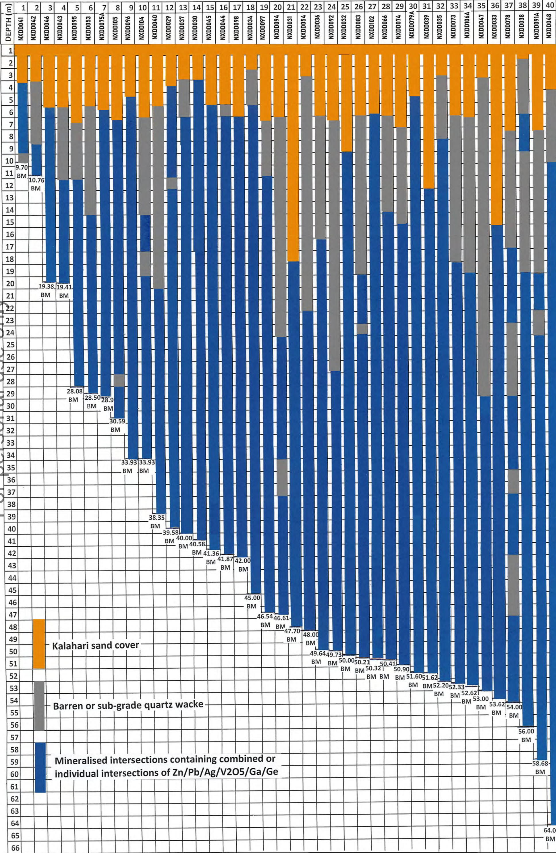
Nxuu Deposit Ga/Ge/V2O5 Mineralisation together with Zn/Pb/Ag Mineralisation
