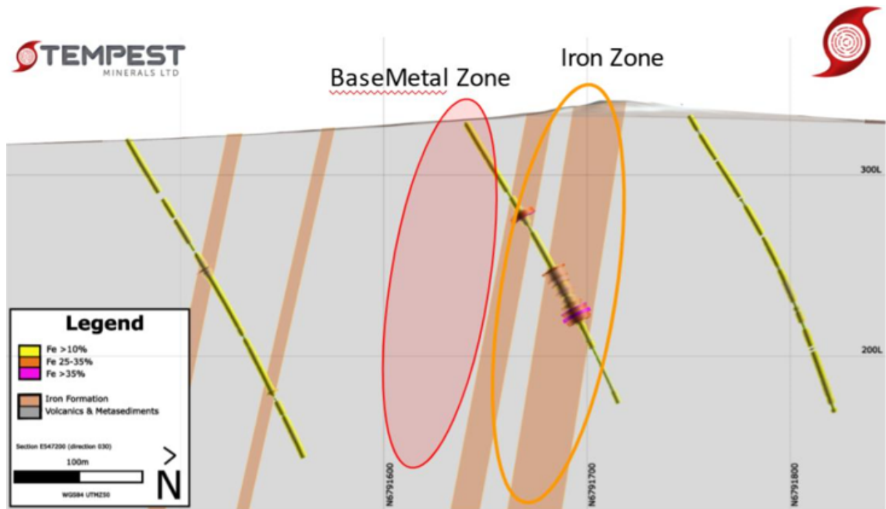
Figure 10: Cross-Section through initial iron mineralisation WARDH160-162
