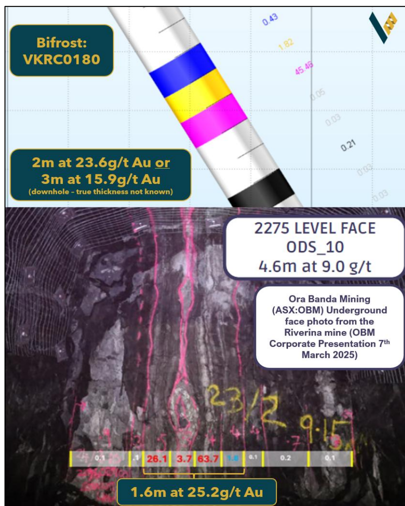
Figure 12; Section through drillhole VKRC0180 drawn at the same scale as underground face photograph taken from the Ora Banda Mining corporate presentation from 7th March 2025. Image illustrates the type and style of mineralisation being explored for by Viking.
