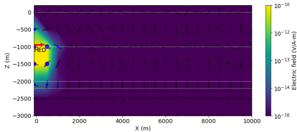
E-field
