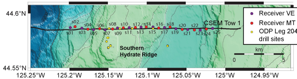
Survey geometry
