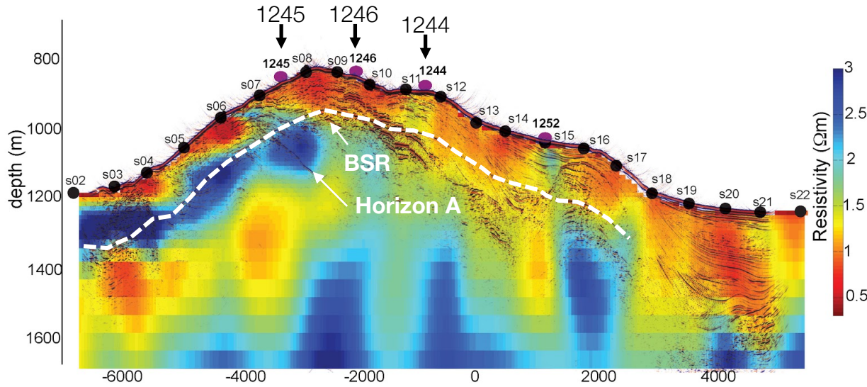
Resistivity section
