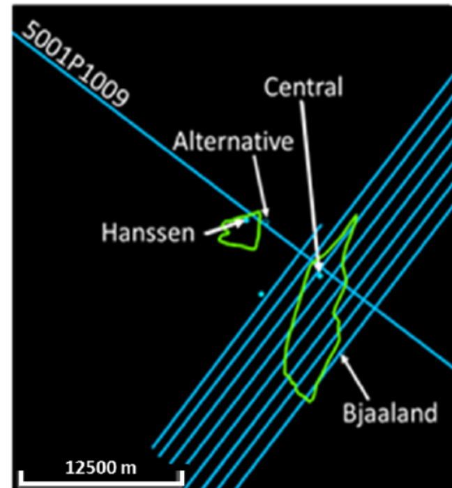
Survey lines
