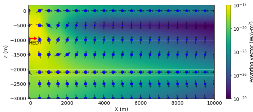
Poynting vector
