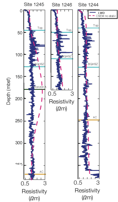
Well-logs
