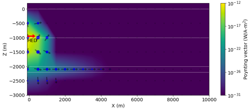
Poynting vector
