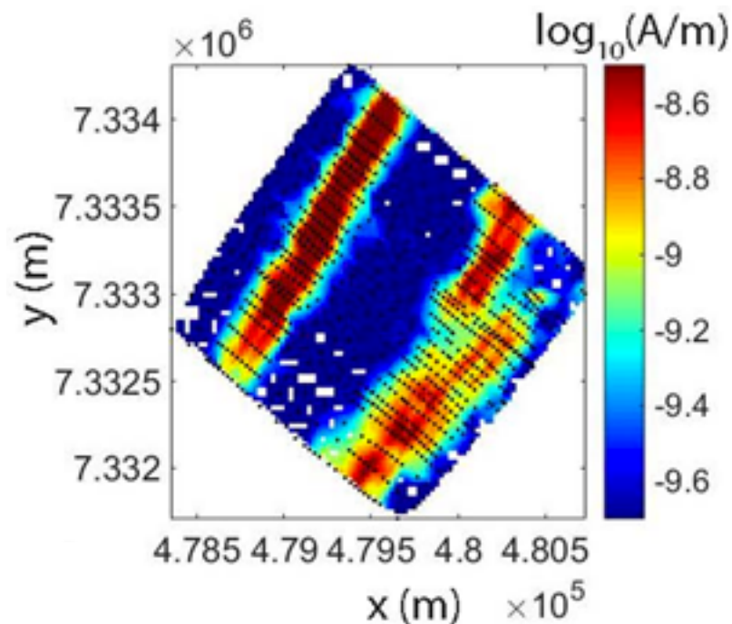
Bz Imaginary at 385 Hz
