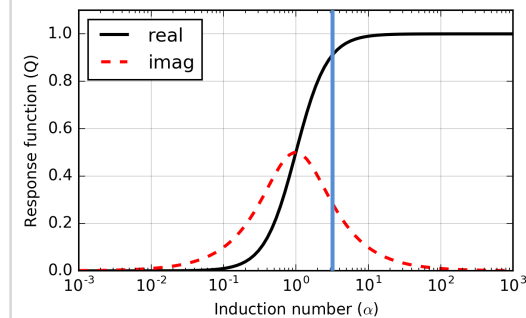
Response curve
