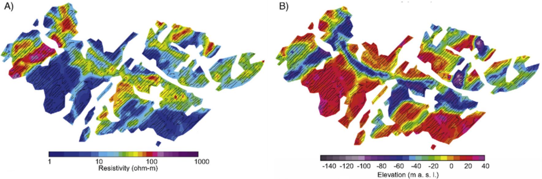
Delineation of valley structures
