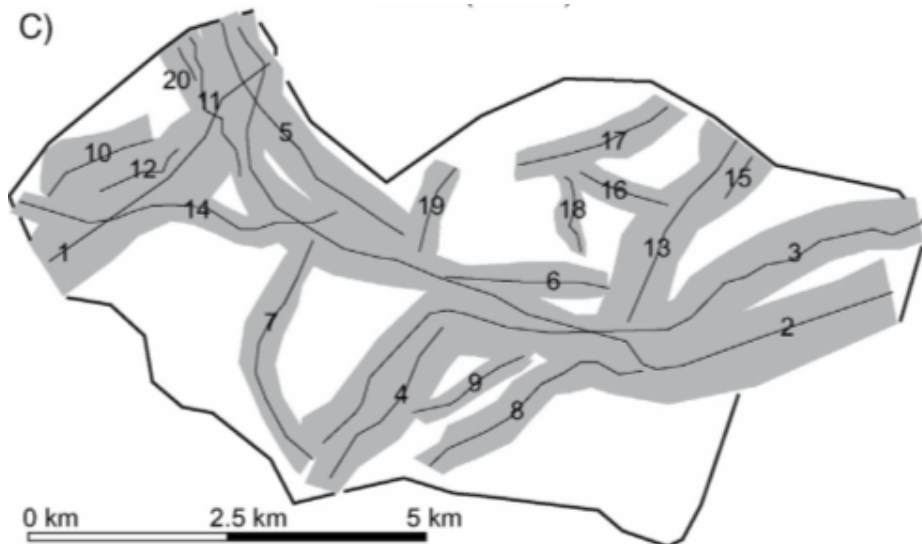
Delineation of valley structures
