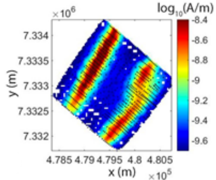
Predicted Bz Imag at 385 Hz
