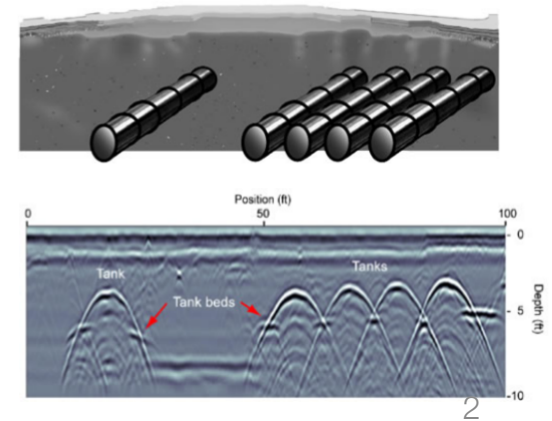
Underground tank
