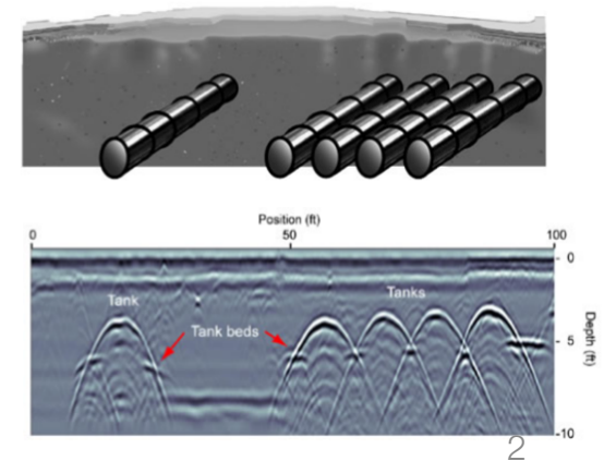
Underground tank
