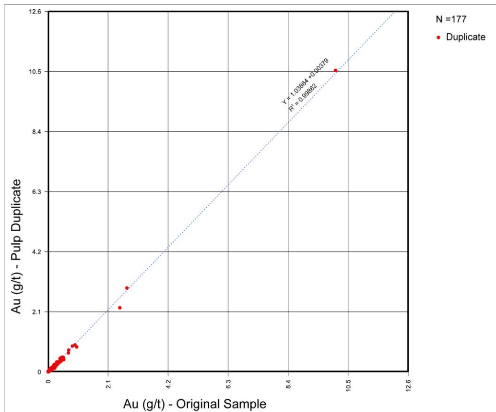
Figure 11-4 : Zoomed in scatterplot with linear trend of pulp duplicates and original samples results from Actlabs for the winter 2020 drilling program (n=177)
