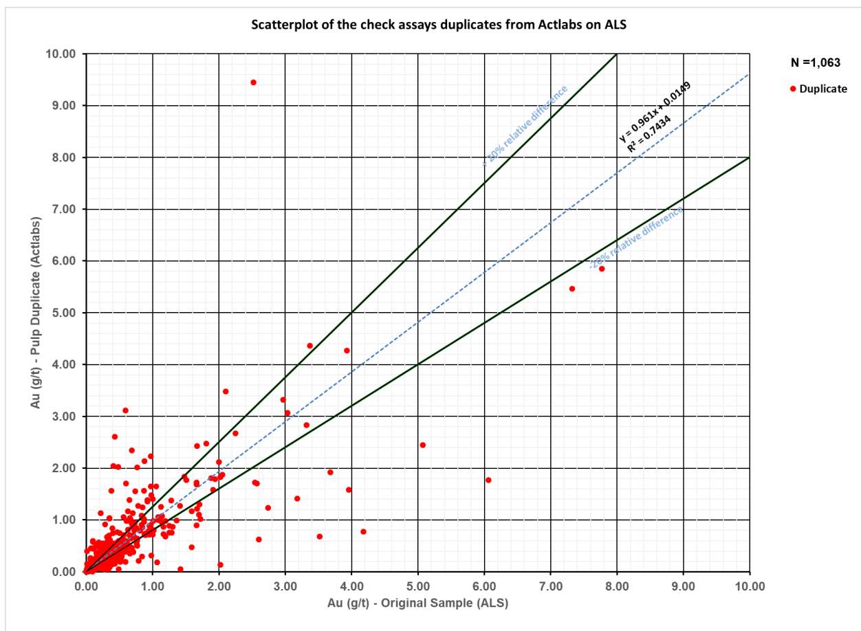
Figure 11-8: Scatterplot of lab check assays duplicates from Actlabs on ALS for the 2013-2019 drilling program (n=1,063) Results above 10 g/t are not shown
