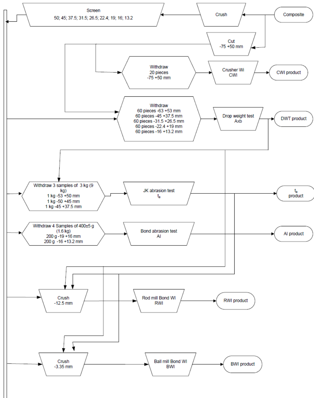
Figure 13-2: COREM comminution testwork protocol
