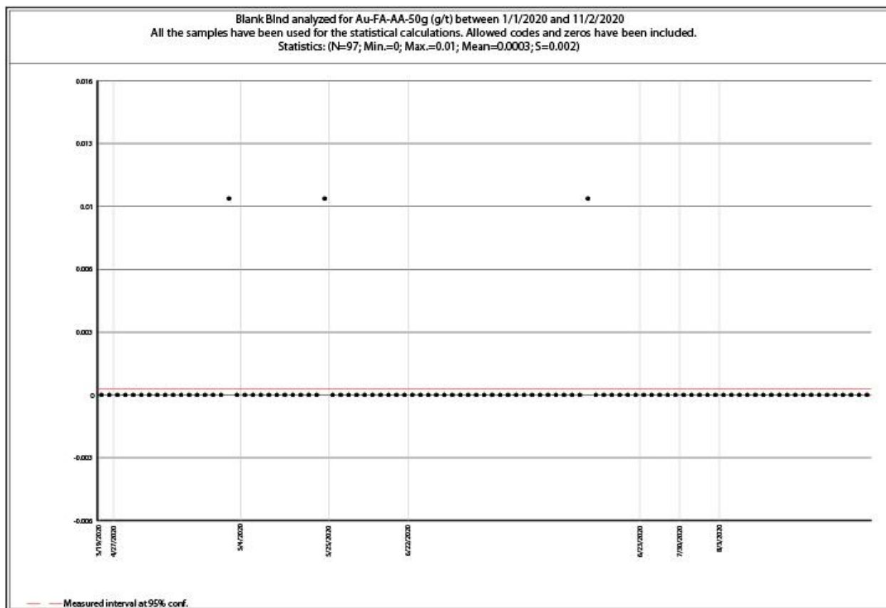
Figure 11-6 : Results for blanks used during the 2020 drilling program (97 samples assayed by Actlabs; detection limit was from 0.005 to 0.01 g/t)
