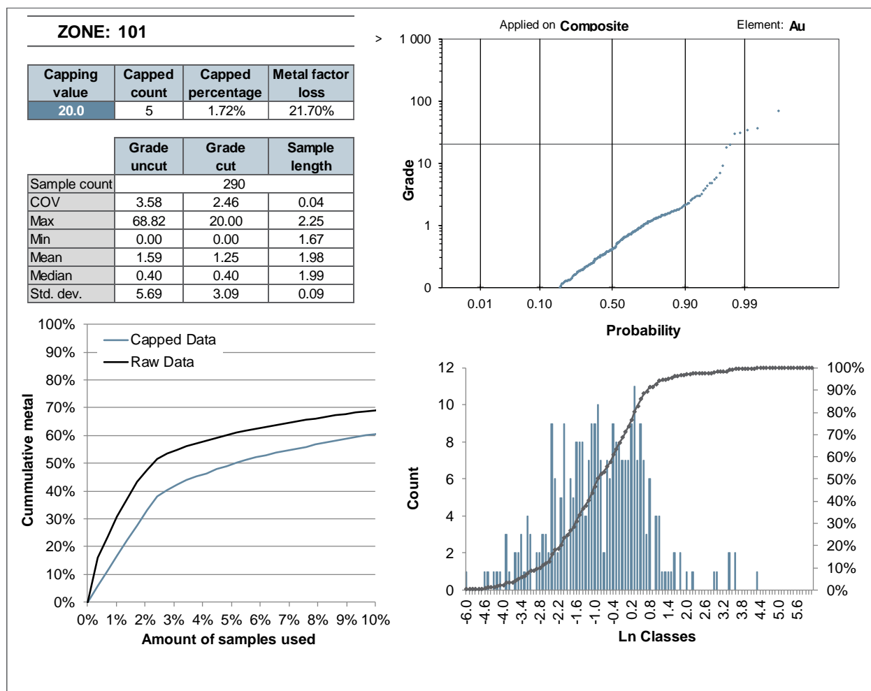
Figure 14-5: Graphs supporting capping threshold decisions on composites for the high-grade mineralized zone 101
