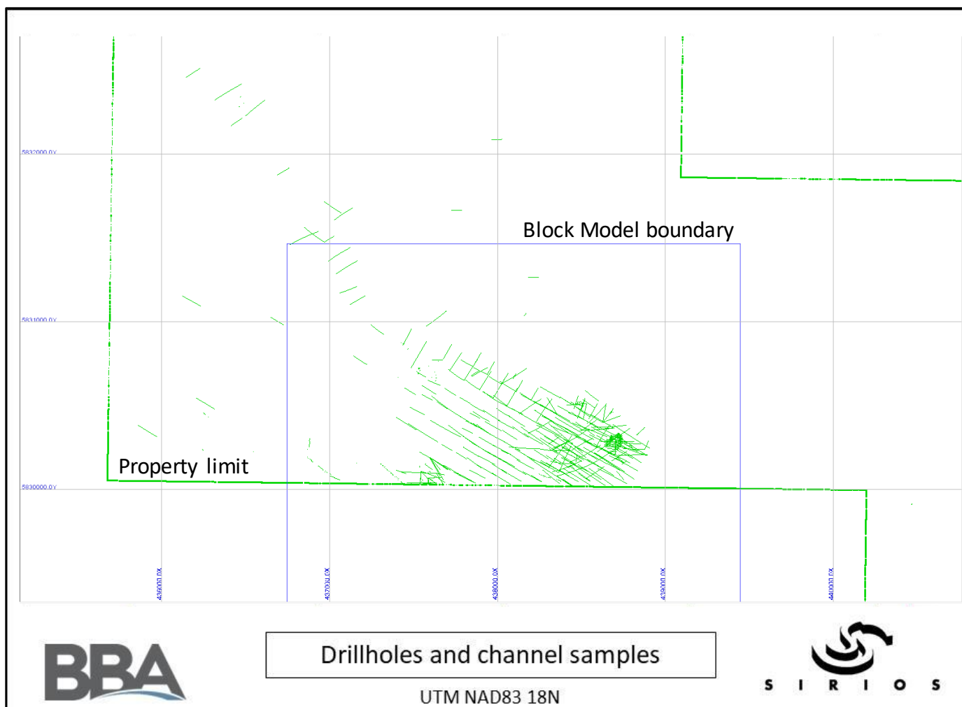
Figure 14-1: 2020 MRE block model, drillholes and channel samples location
