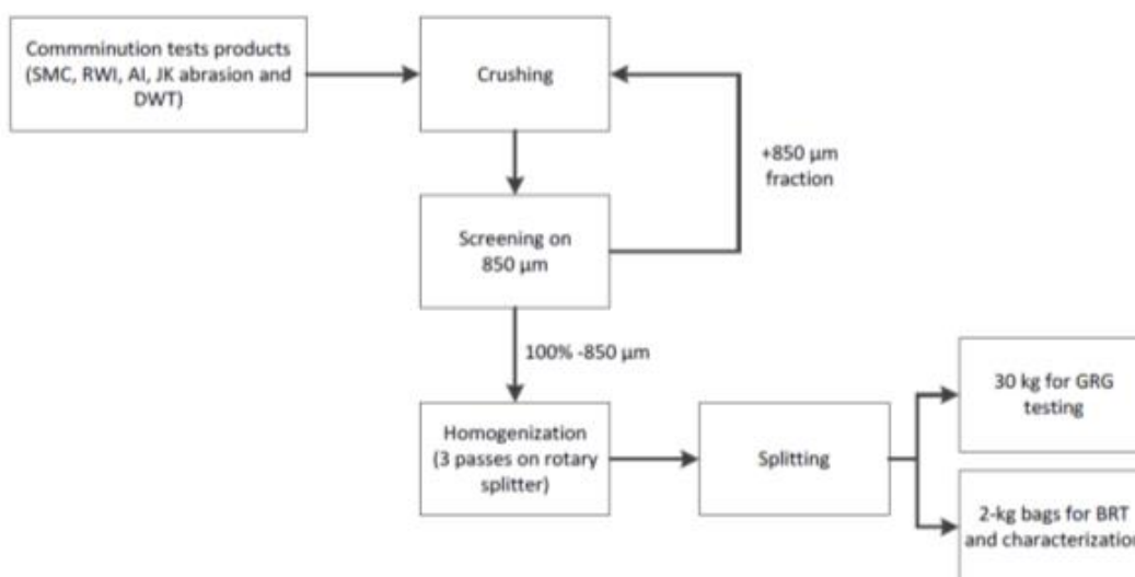
Figure 13-3: COREM metallurgical samples preparation flow diagram
