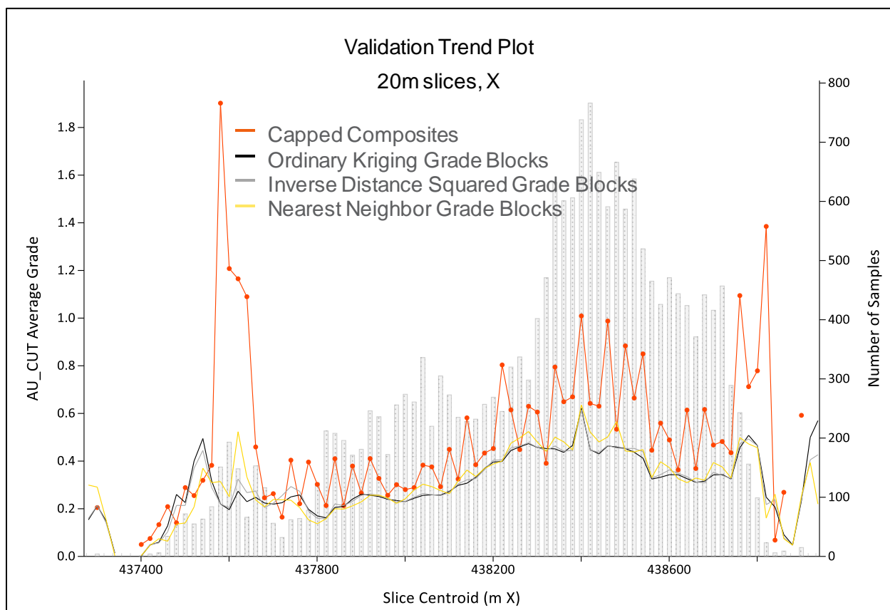
Figure 14-18: Block model validation swath plot along strike (X-direction)
