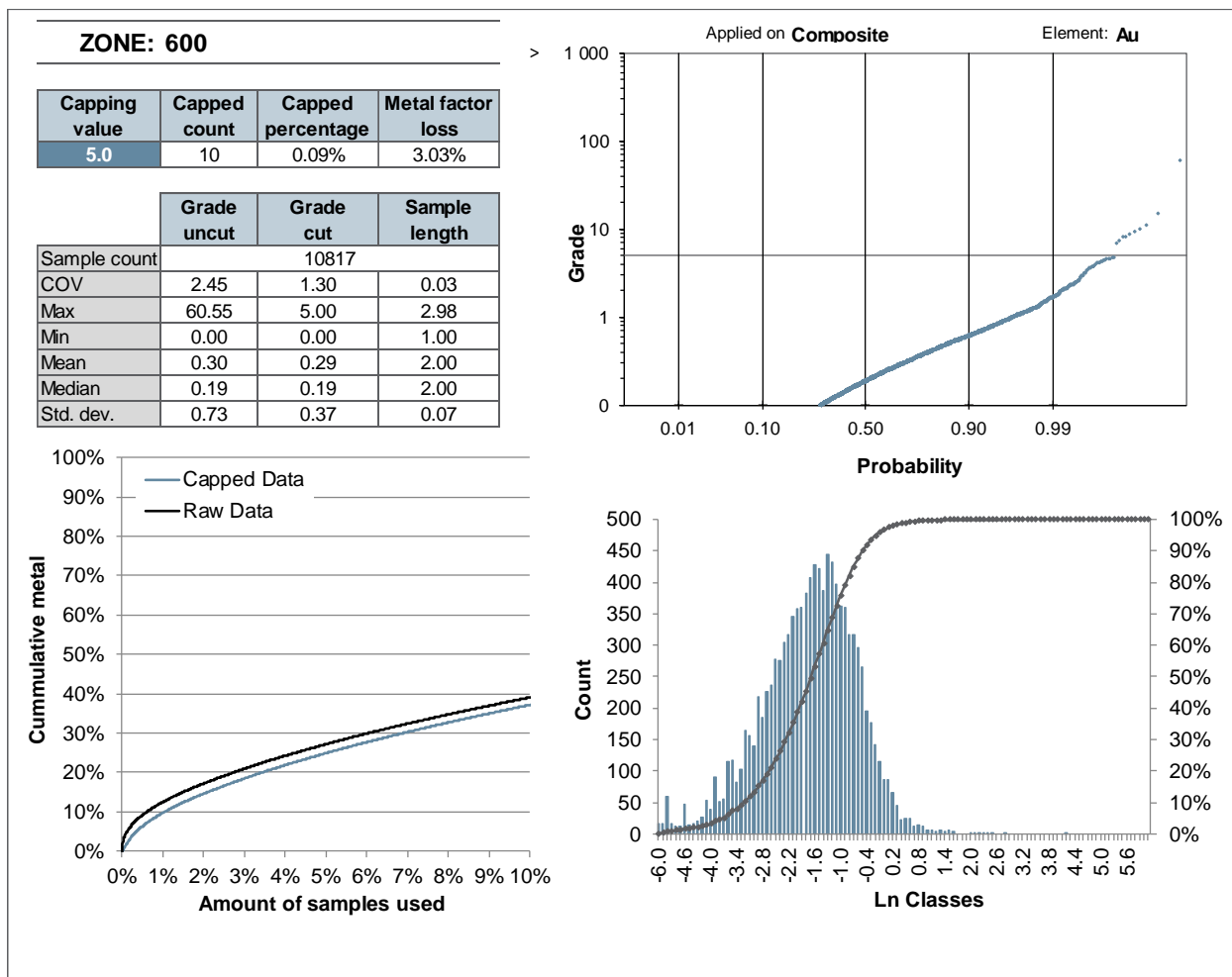
Figure 14-10: Graphs supporting capping threshold decisions on composites for the low-grade domain 600
