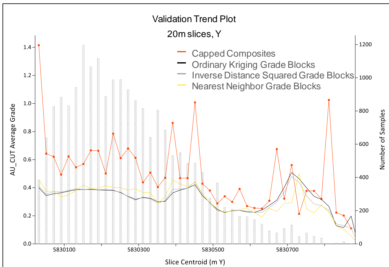
Figure 14-19: Block model validation swath plots across strike (Y-direction)
