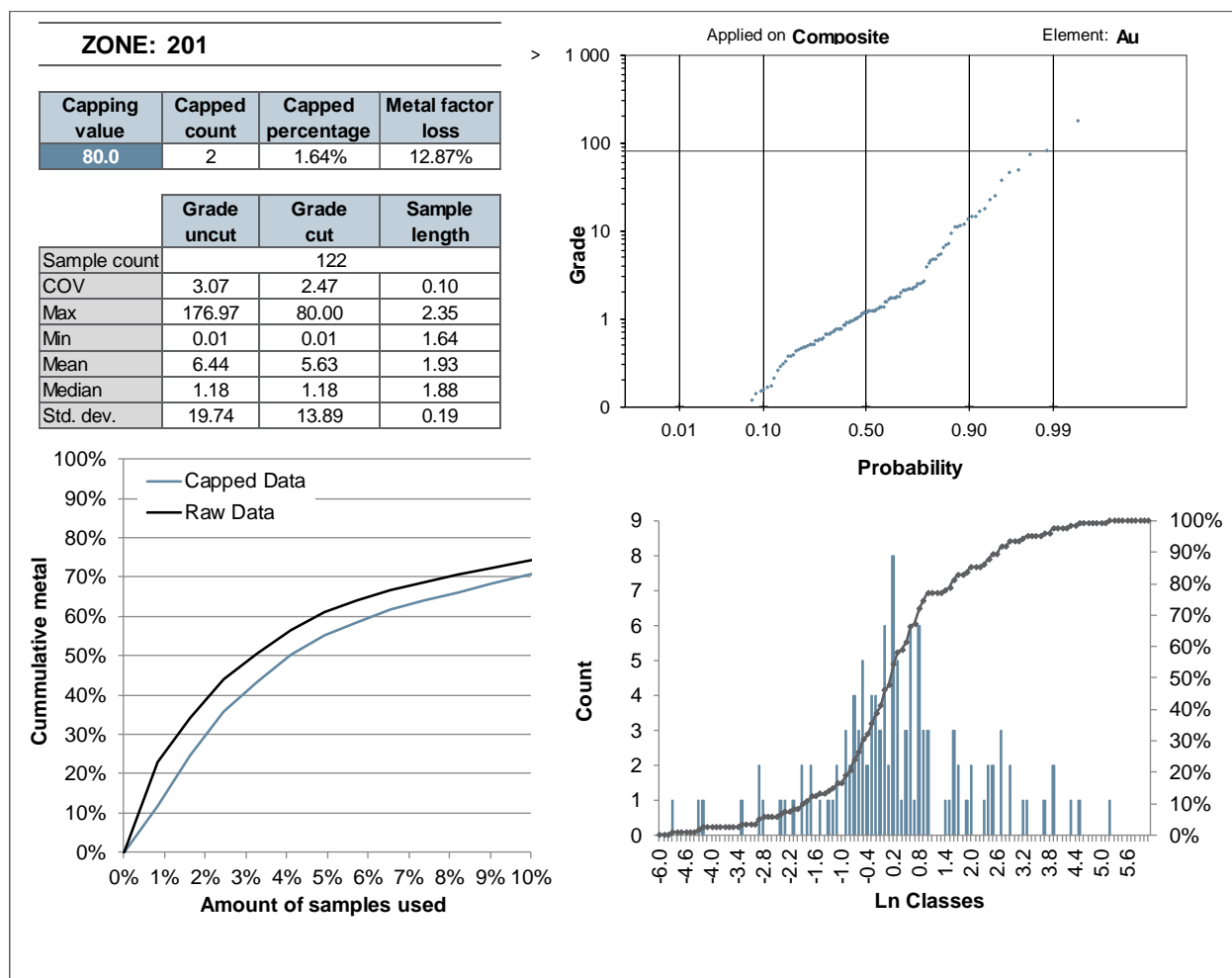
Figure 14-7: Graphs supporting capping threshold decisions on composites for the high-grade mineralized zone 201
