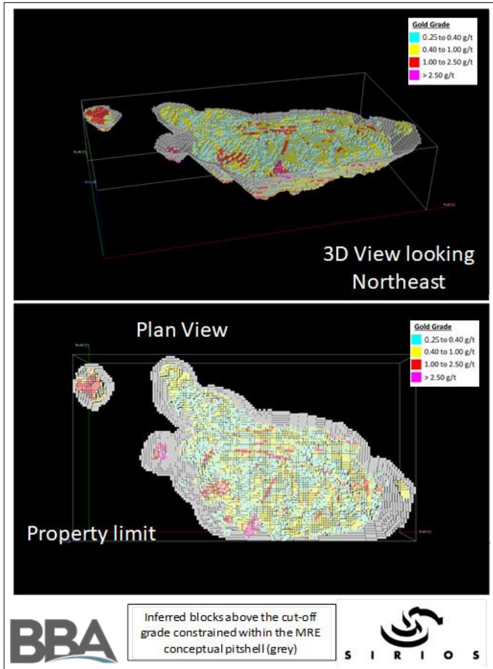
Figure 14-21: 3D and Plan views showing grade distribution and classification of the Project above the cut-off grade
