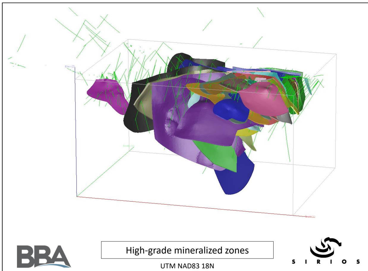
Figure 14-2: 3D view looking north-northwest (NNW) of the high-grade mineralized zones and of the drillholes included in this resource estimate Note that the X-axis is 1,800 m in length.
