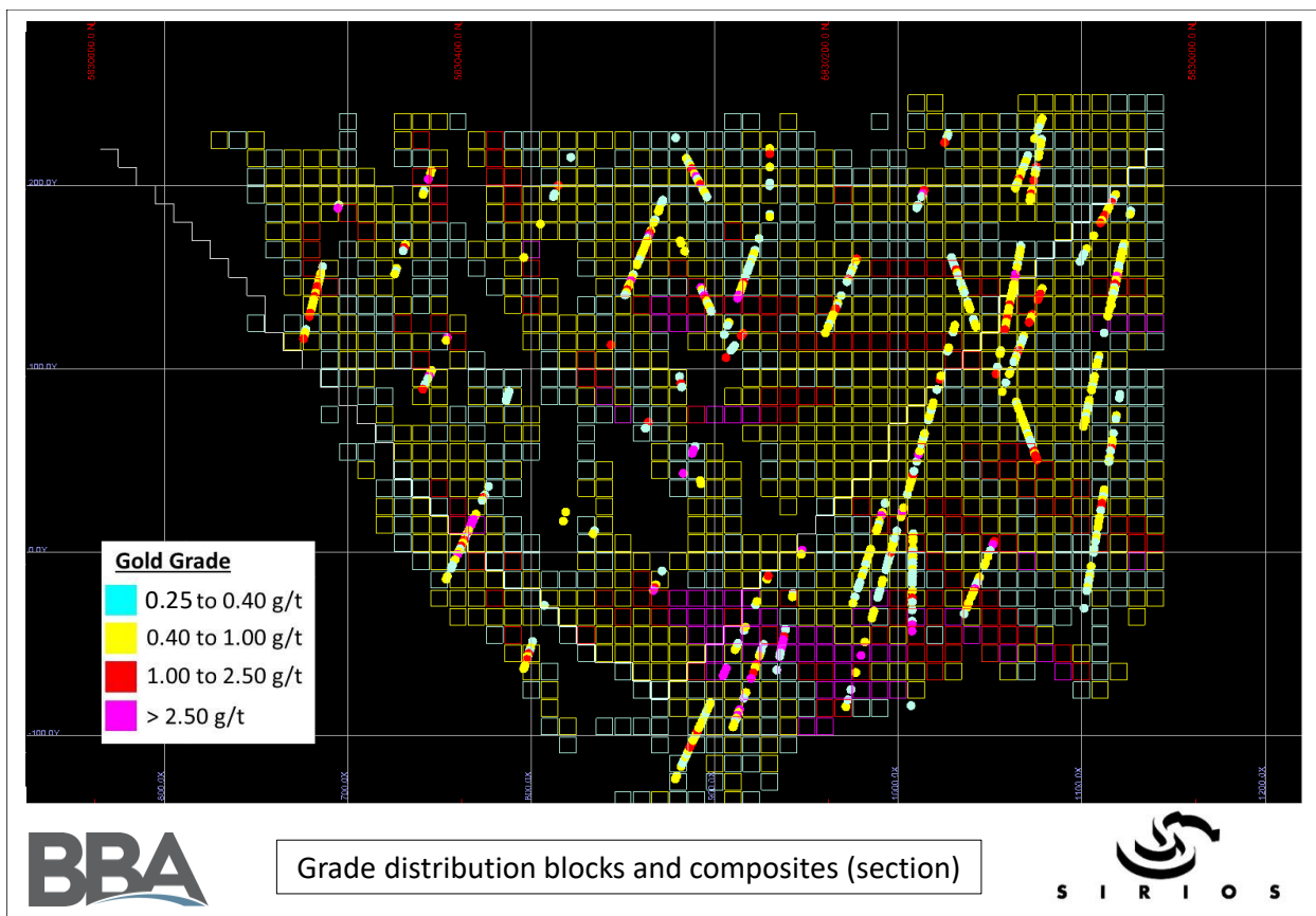
Figure 14-16: Comparative example of the grade distribution between the blocks and the composites in section view
