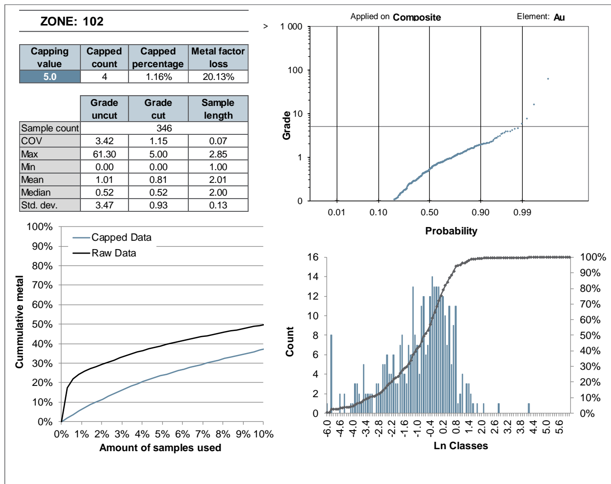
Figure 14-6: Graphs supporting capping threshold decisions on composites for the high-grade mineralized zone 102
