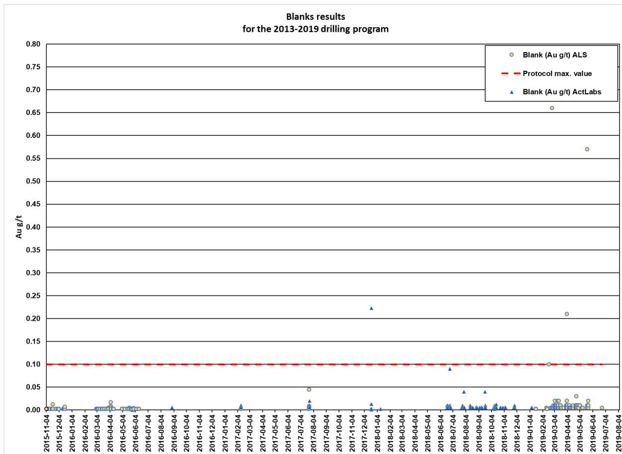
Figure 11-5: Results for blanks used during the 2013-2019 drilling program
