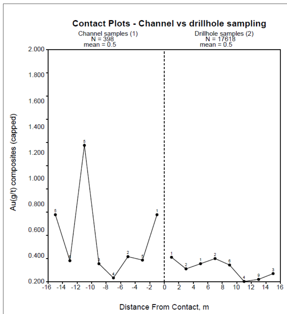
Figure 14-13: Contact analysis on the capped composites between the channel and the drillholes data
