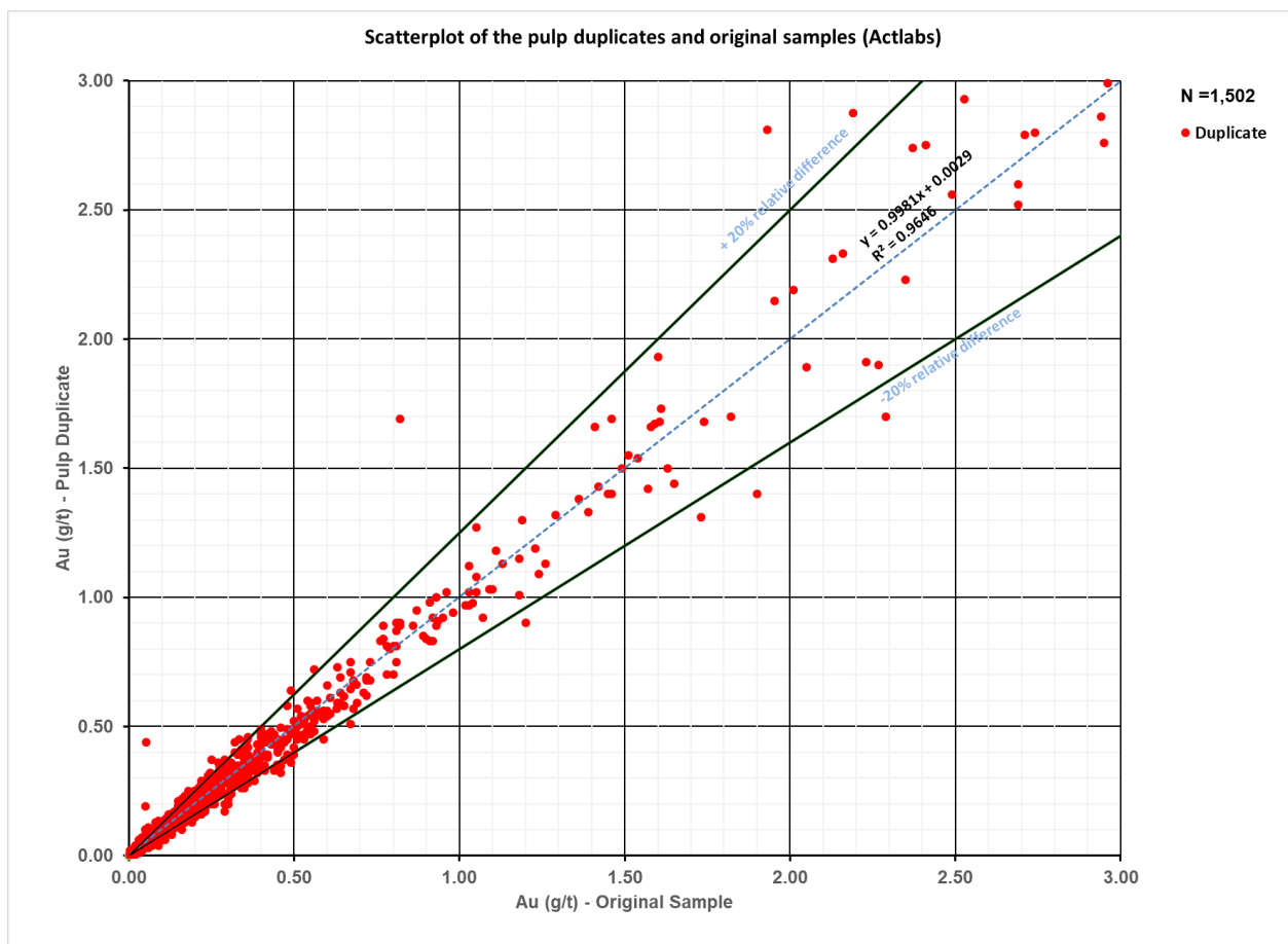
Figure 11-3: Zoomed in scatterplot with linear trend of pulp duplicates and original samples results from Actlabs for the 2013-2019 drilling program (n=1,502) (22 higher grade results are not shown)
