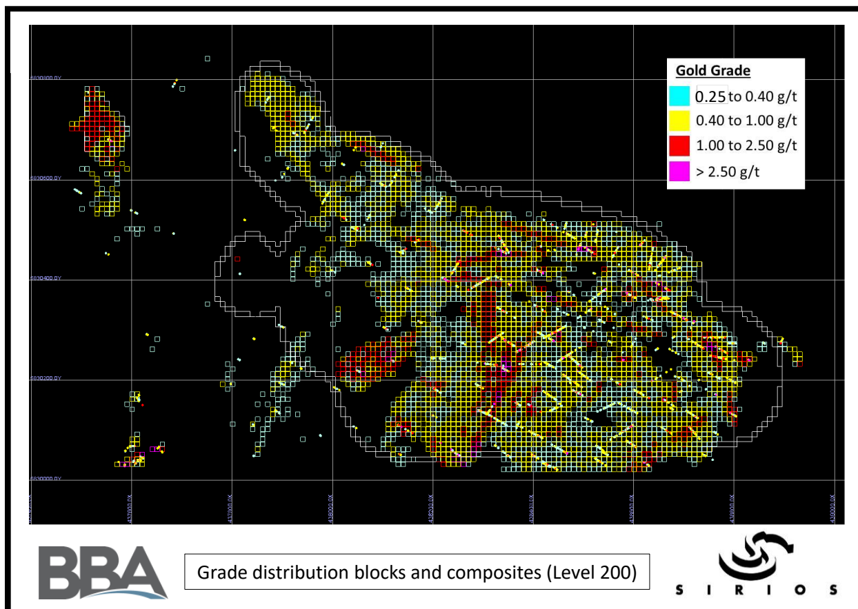
Figure 14-17: Comparative example of the grade distribution between the blocks and the composites in plan view (Level 200)
