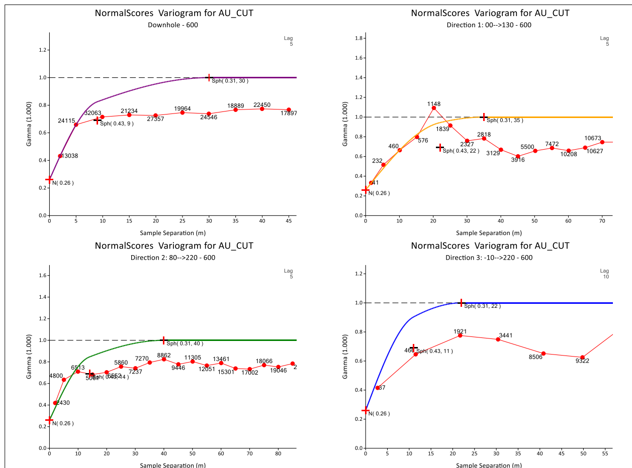
Figure 14-12: Example of the variography study for the low-grade domain 600
