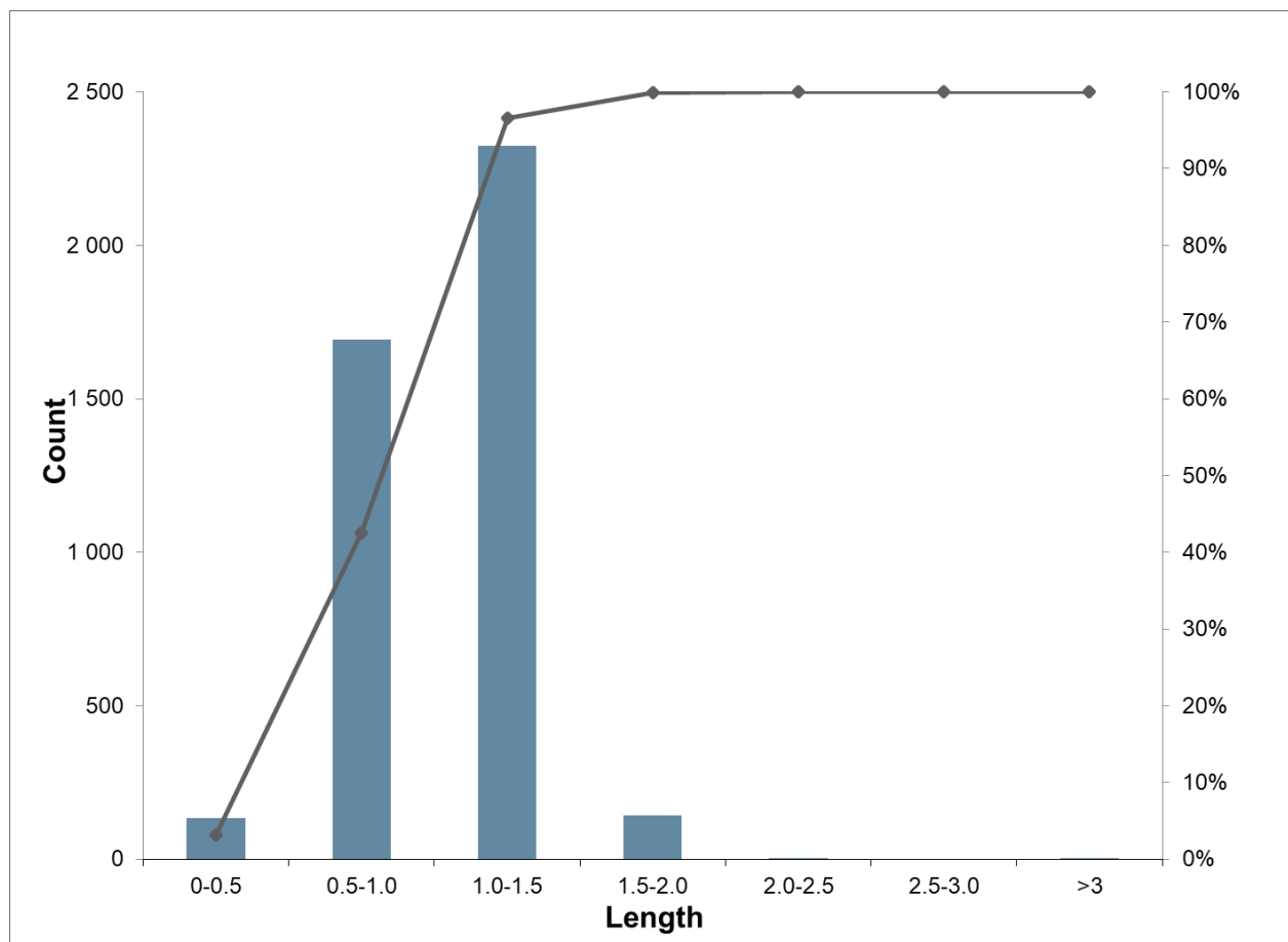
Figure 14-4: Sample length distribution within the high-grade domains
