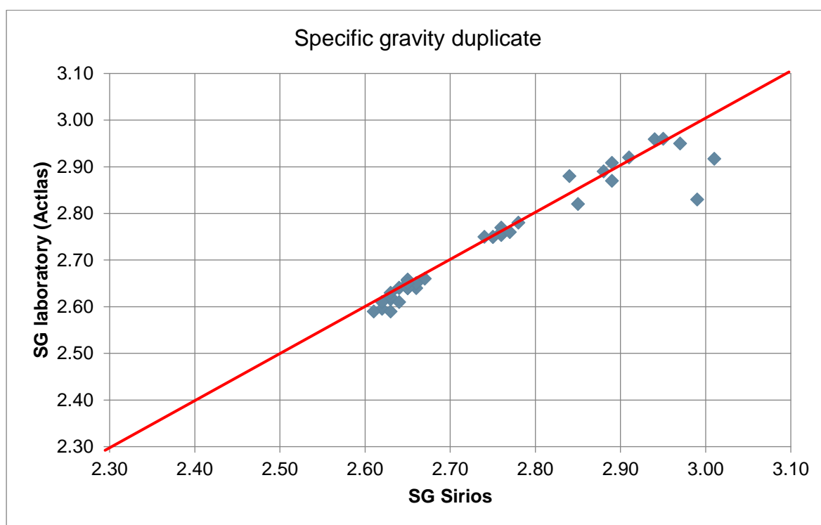
Figure 11-1: Specific gravity measured by Sirios vs specific gravity measured by Actlabs
