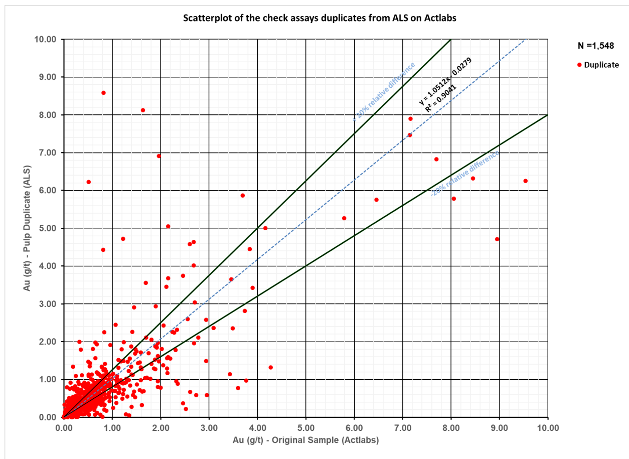
Figure 11-7: Scatterplot of lab check assays duplicates from ALS on Actlabs for the 2013-2019 drilling program (n=1,548) (results above 10 g/t are not shown)
