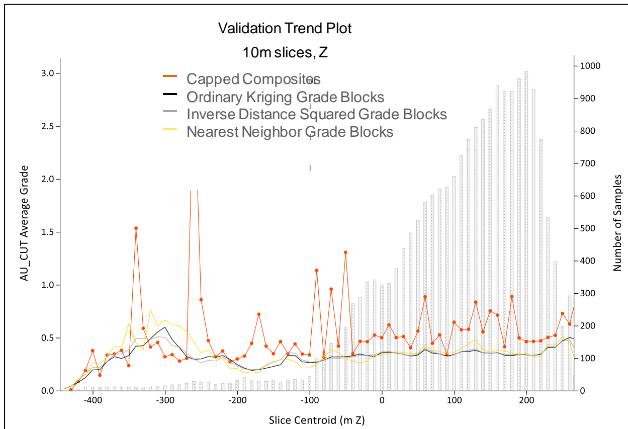
Figure 14-20: Block model validation swath plots along elevation (Z-direction)
