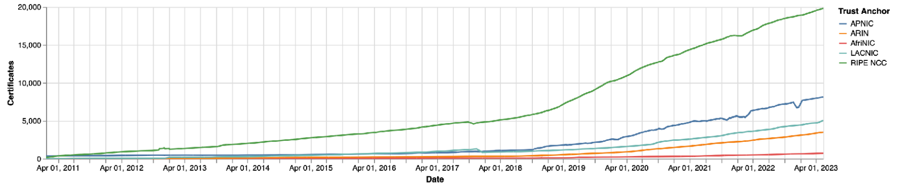
IPv4 address space in ROAs (/24s)
