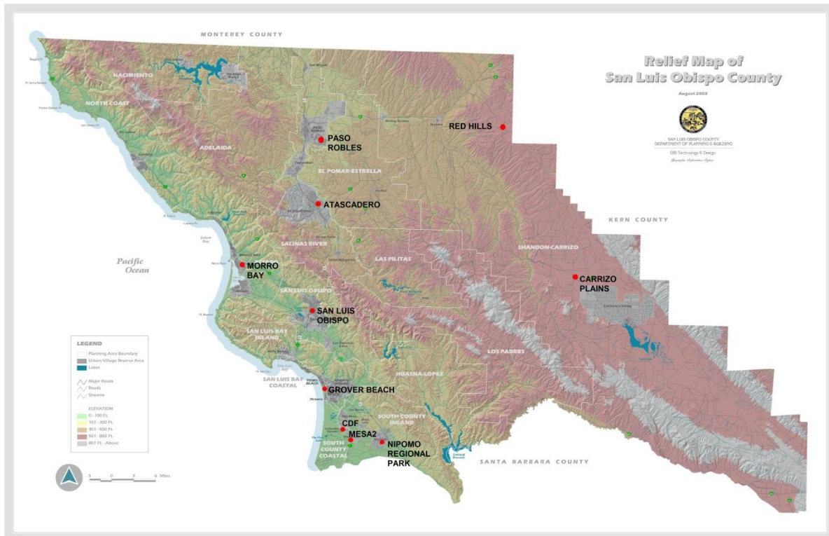
Figure 1: Map of Ambient Air Monitoring Stations in San Luis Obispo County in 2011
