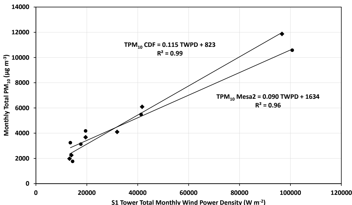
Figure 2-27. Relation Between TPM 10 (μg m -3 ) and TWPD (W m -2 ) at SLOAPCD CDF and Mesa2 Monitoring Stations
