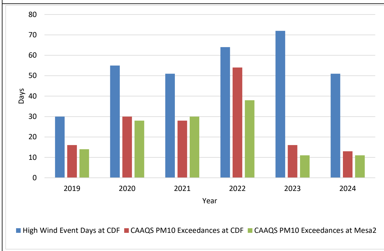
Figure 2-33. High Wind Event Days at the CDF Air Quality Monitoring Station and 24-Hour Average PM 10 CAAQS Exceedances at the CDF and Mesa2 Air Quality Monitoring Stations, Approximately January through July, 2019 to 2024
