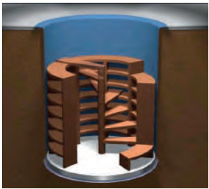
Stapelen van de beton elementen. Installing the construction components.
