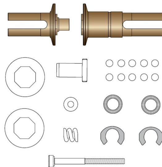
FXX Alum. ball diff. FXX 鋁合金滾珠差速器 210353
