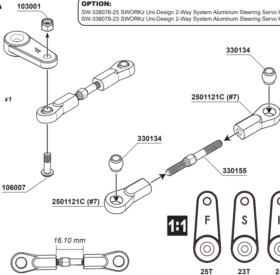
330155 Steering Servo Turnbuckle (M3x30mm) x1
