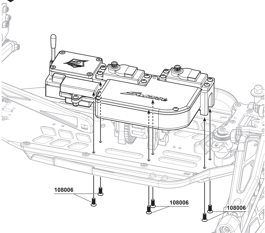
108006 M3x8mm FH/ST HEX Screw x6
