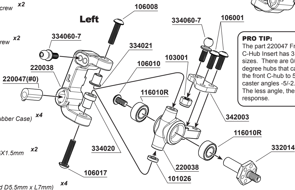
332014 Steering Hub Hinge Pin x2
