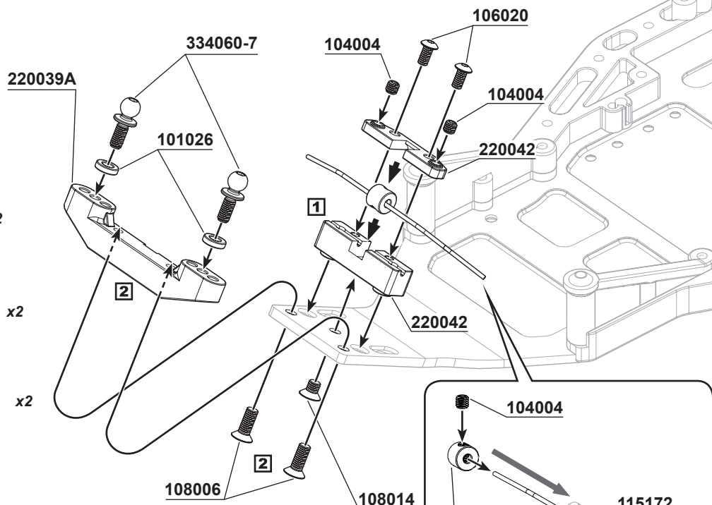
106020 M2.5x5mm Hex Socket OH/TP Screw x2
