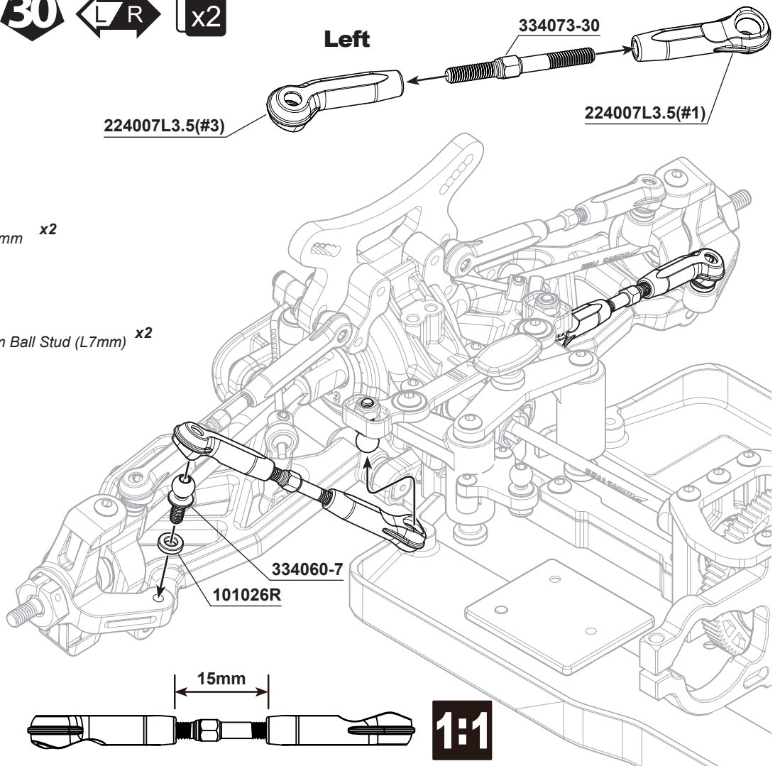
334073-30 Steering Servo Turnbuckle x2
