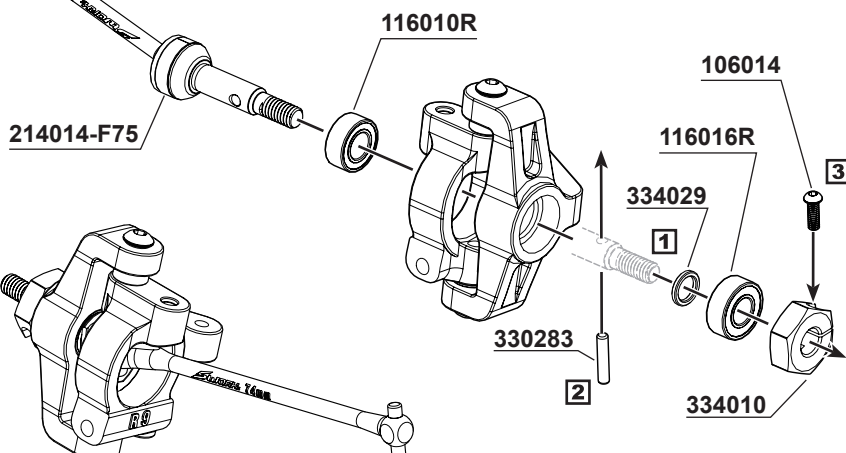
214014-F75 S14-4 Axle Universal Cross Drive Shaft Set 75mm x2
