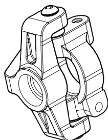
220024-9 SWORKz 1/10 S14-3 Front C Hub Set (9 Degree) 220024-11 SWORKz 1/10 S143C Front C Hub Set (11 Degree)
