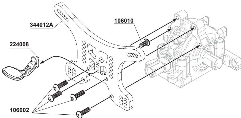
106002 M3x10mm Hex Socket OH/TP Screw x4
