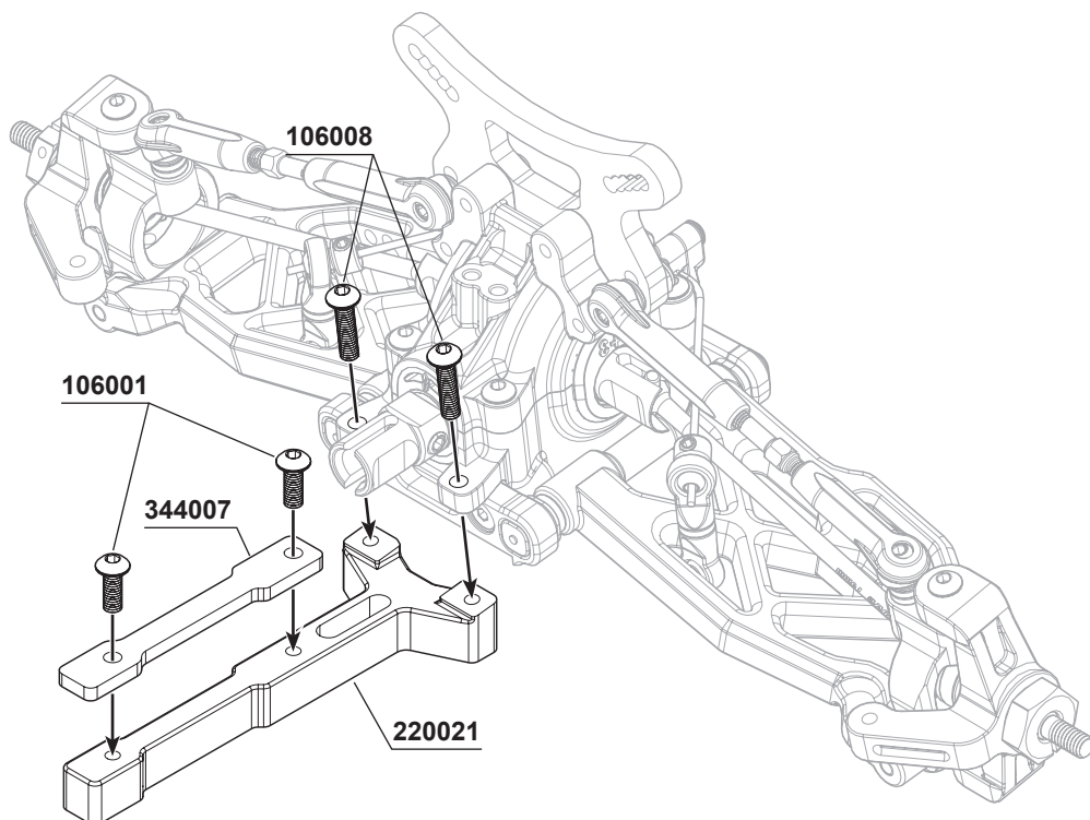
106008 M3x12mm Hex Soked OH/TP Screw
