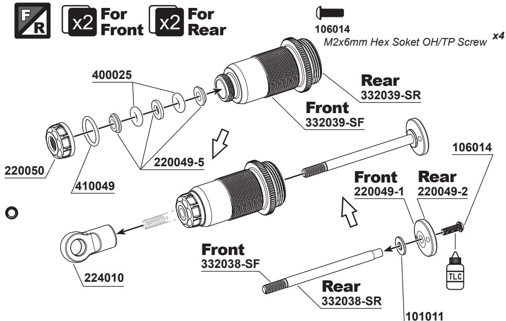
220049-5 Shock seal washer 3.0x6.5x2.0mm x8
