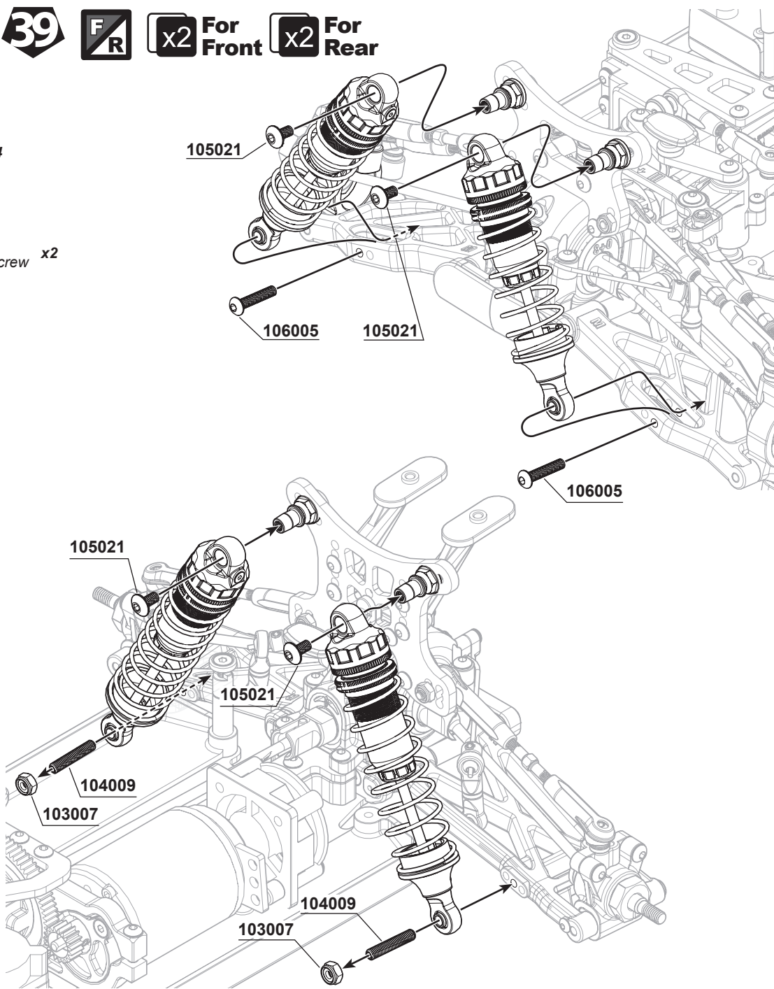
105021 M3x6mm Taper head screw
