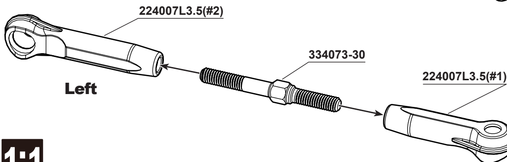
334073-30 Steering Servo Turnbuckle x2
