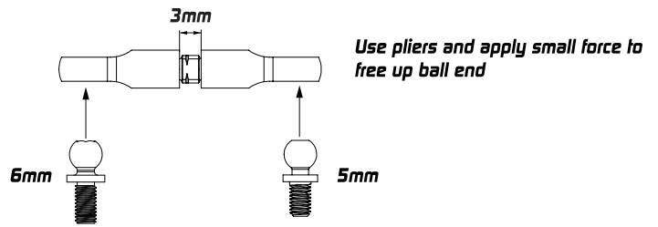
For Rear Camber Link
