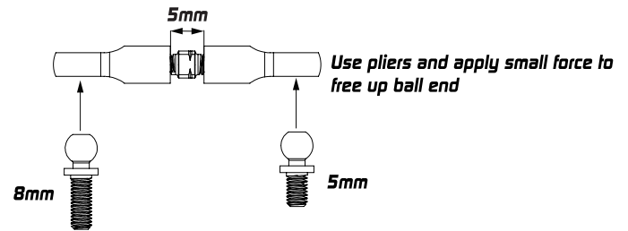
For Front Camber Link
