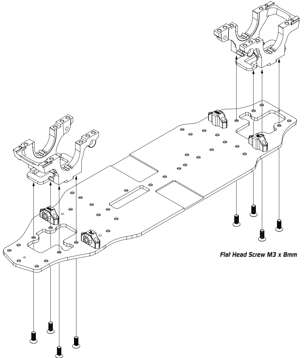
Flat Head Screw M3 x 8mm
