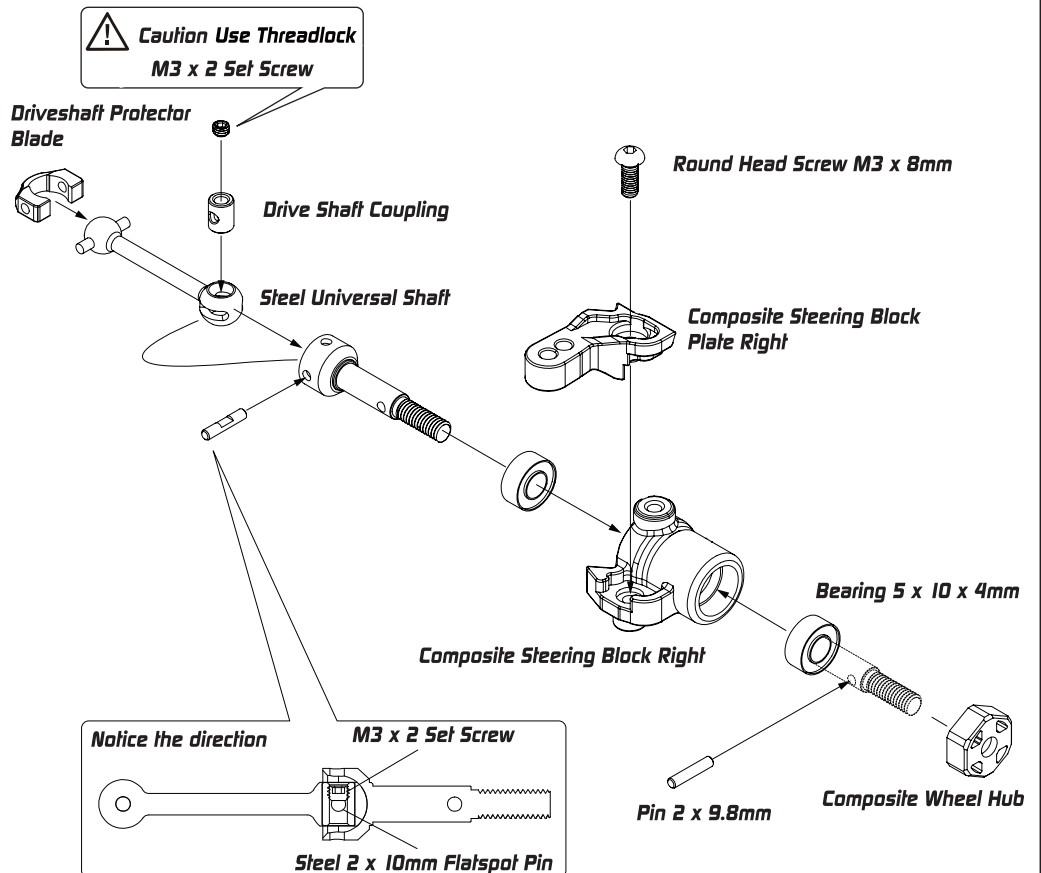
Round Head Screw RM3 x 8mm XP-40038
