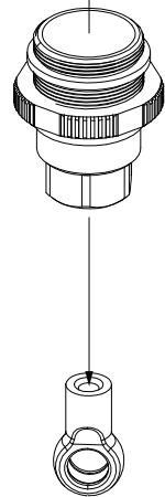
Shock Lower Connector
