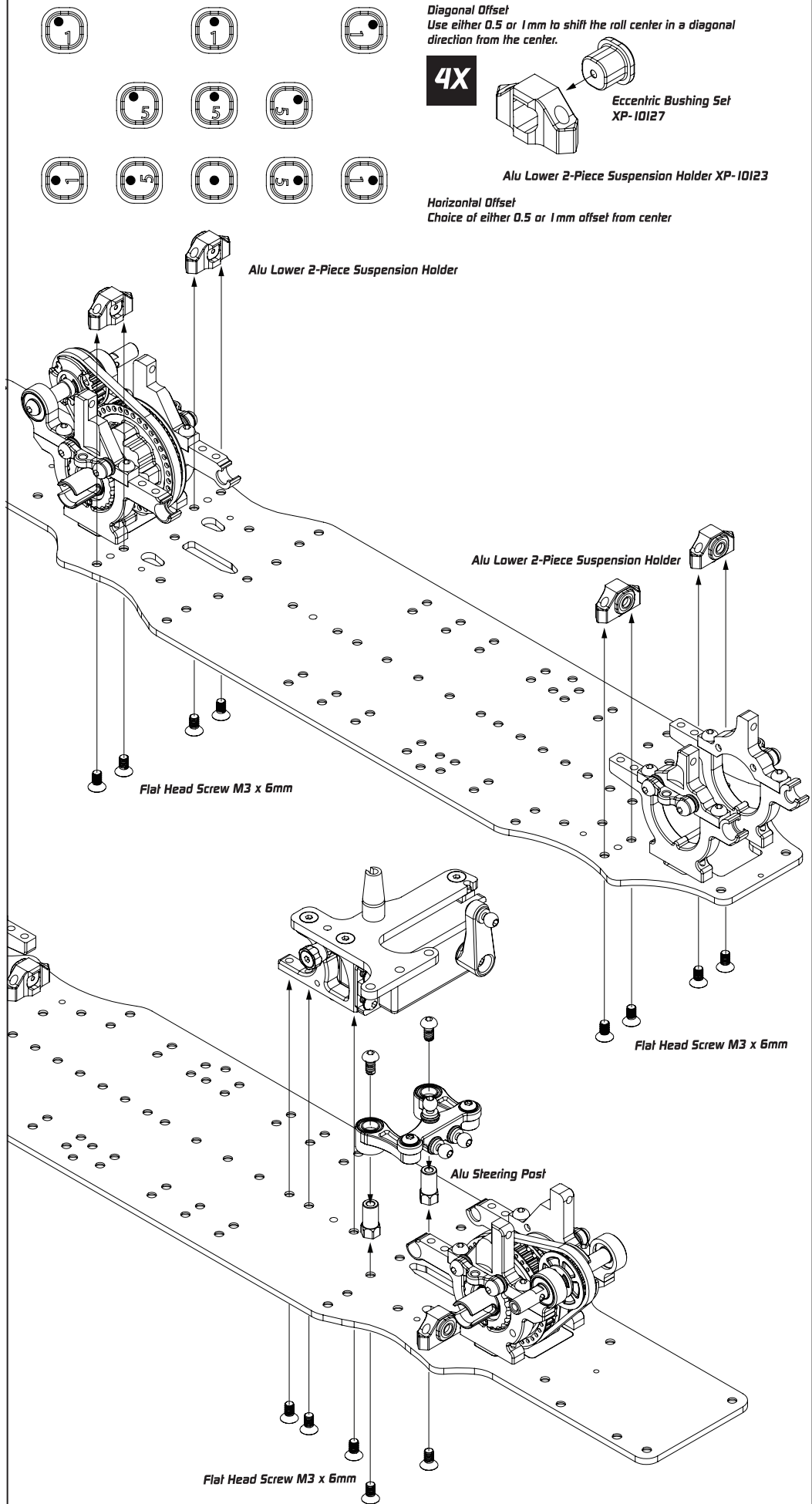
Alu Steering Post For Dual Servo Saver 11.5mm XP-10494
