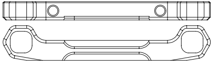
Alu Rear Lower I-Piece Suspension holder - RR XP-10124
