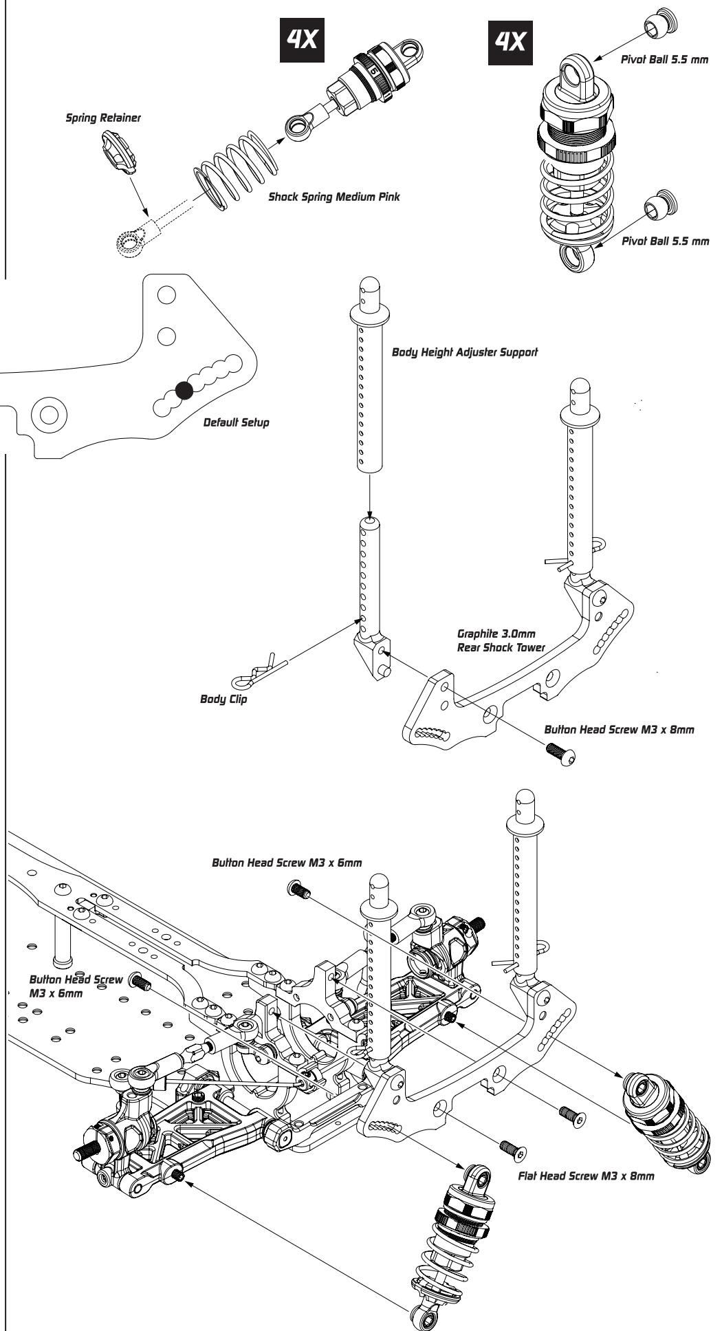
Graphite 3.0mm Rear Shock Tower XP-10574
