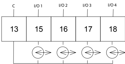
4 Configurable inputs/outputs
