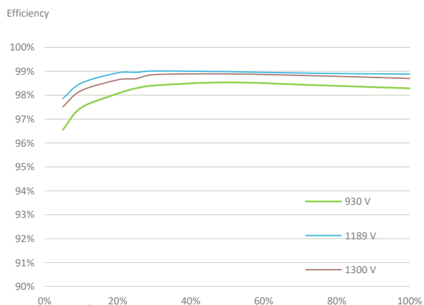
Efficiency Curve
