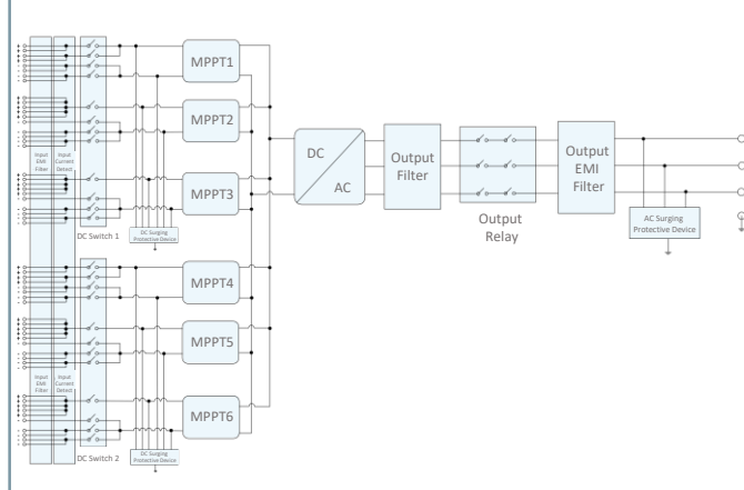
Circuit Diagram
