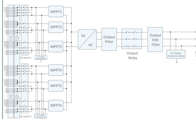
Circuit Diagram
