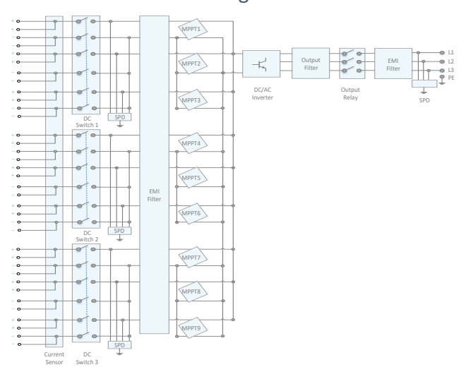
Circuit Diagram
