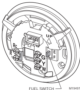
Fig. 7. Fuel switch.
