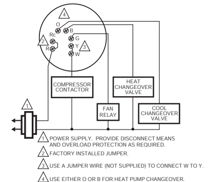
Fig. 6. Typical hookup of T8775C in single-stage heat pump system.
