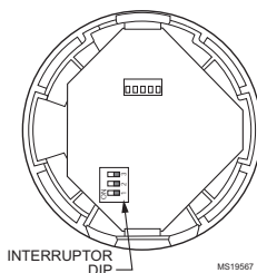
Fig. 8. Interruptor DIP.
