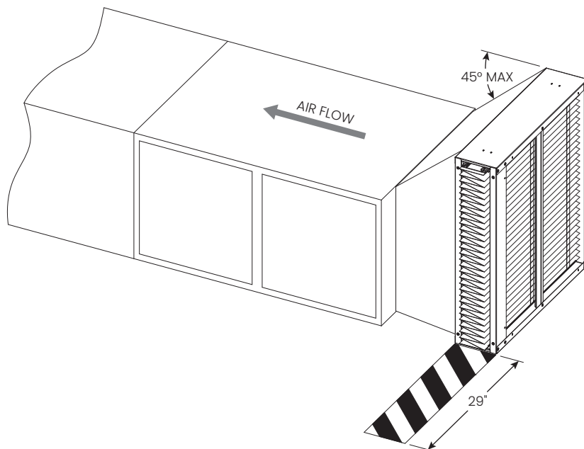
FIGURE 1: TYPICAL APPLICATION OF THE AIR CLEANER MOUNTED TO A HORIZONTAL SYSTEM
