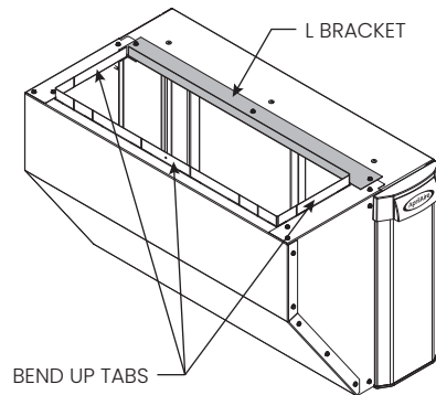
FIGURE 4: 8" x 24" OFFSET LEFT
